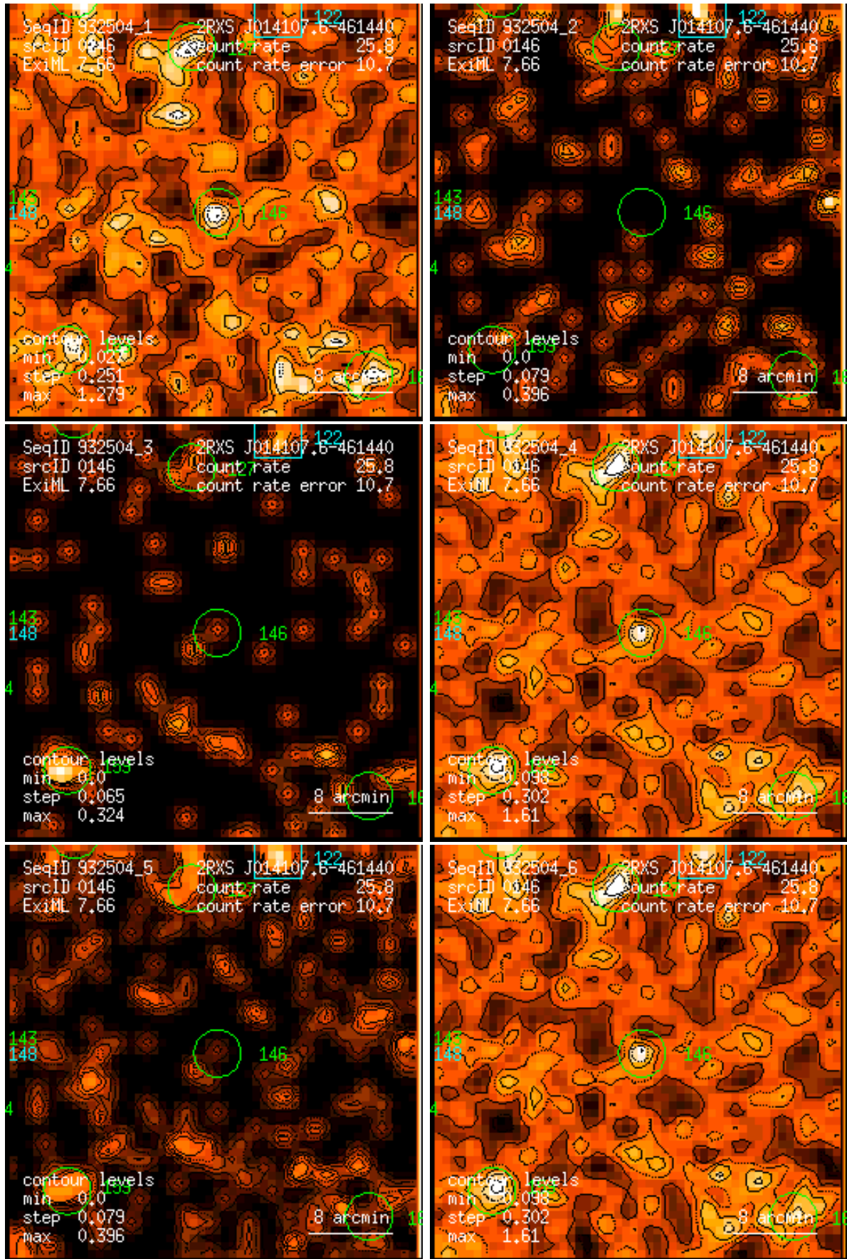
Figure 146: RASS 932504: detection 0146: band rate images, Gaussian filter: (1) PSPC channels 11 – 41, (2) 52 – 90, (3) 91 – 201, (4) 11 – 235, (5) 52 – 201, (6) 11 – 201. Broad band rates in counts/ks. Band rate contour levels in counts/ks/arcmin 2 .
