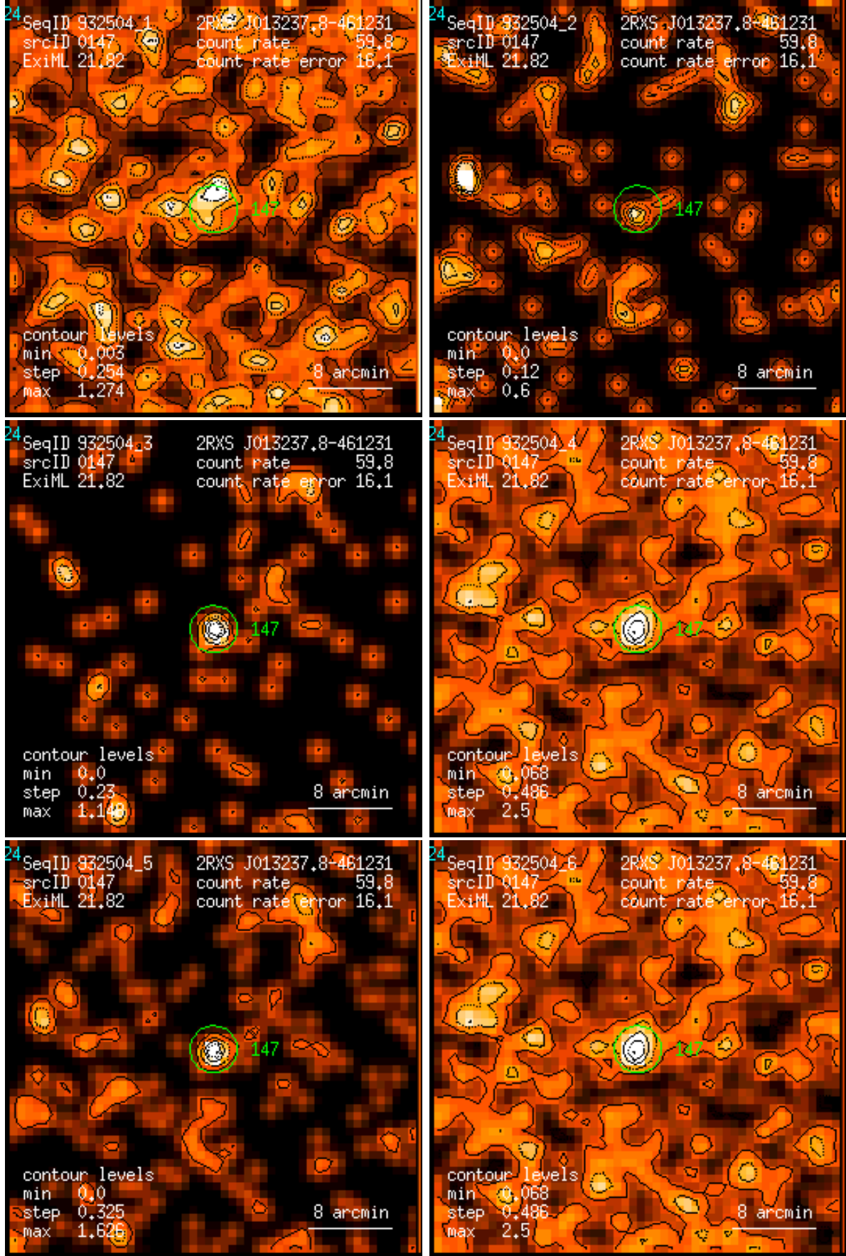
Figure 147: RASS 932504: detection 0147: band rate images, Gaussian filter: (1) PSPC channels 11 – 41, (2) 52 – 90, (3) 91 – 201, (4) 11 – 235, (5) 52 – 201, (6) 11 – 201. Broad band rates in counts/ks. Band rate contour levels in counts/ks/arcmin 2 .
