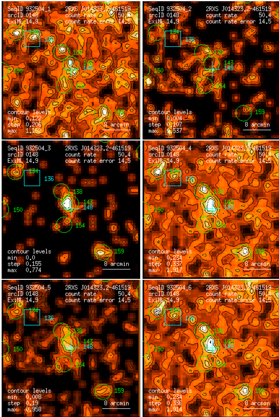
Figure 148: RASS 932504: detection 0148: band rate images, Gaussian filter: (1) PSPC channels 11 – 41, (2) 52 – 90, (3) 91 – 201, (4) 11 – 235, (5) 52 – 201, (6) 11 – 201. Broad band rates in counts/ks. Band rate contour levels in counts/ks/arcmin 2 .
