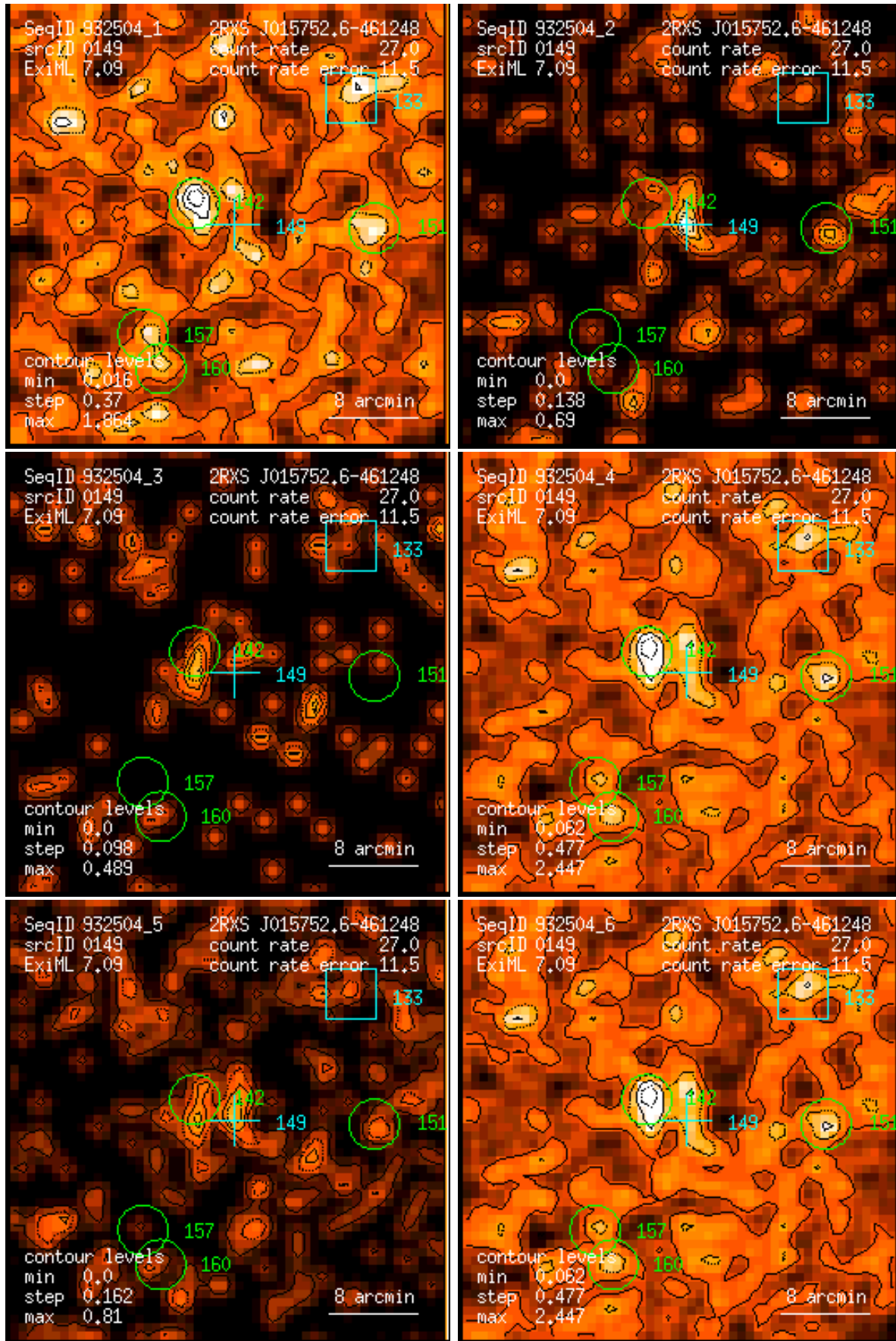
Figure 149: RASS 932504: detection 0149: band rate images, Gaussian filter: (1) PSPC channels 11 – 41, (2) 52 – 90, (3) 91 – 201, (4) 11 – 235, (5) 52 – 201, (6) 11 – 201. Broad band rates in counts/ks. Band rate contour levels in counts/ks/arcmin 2 .
