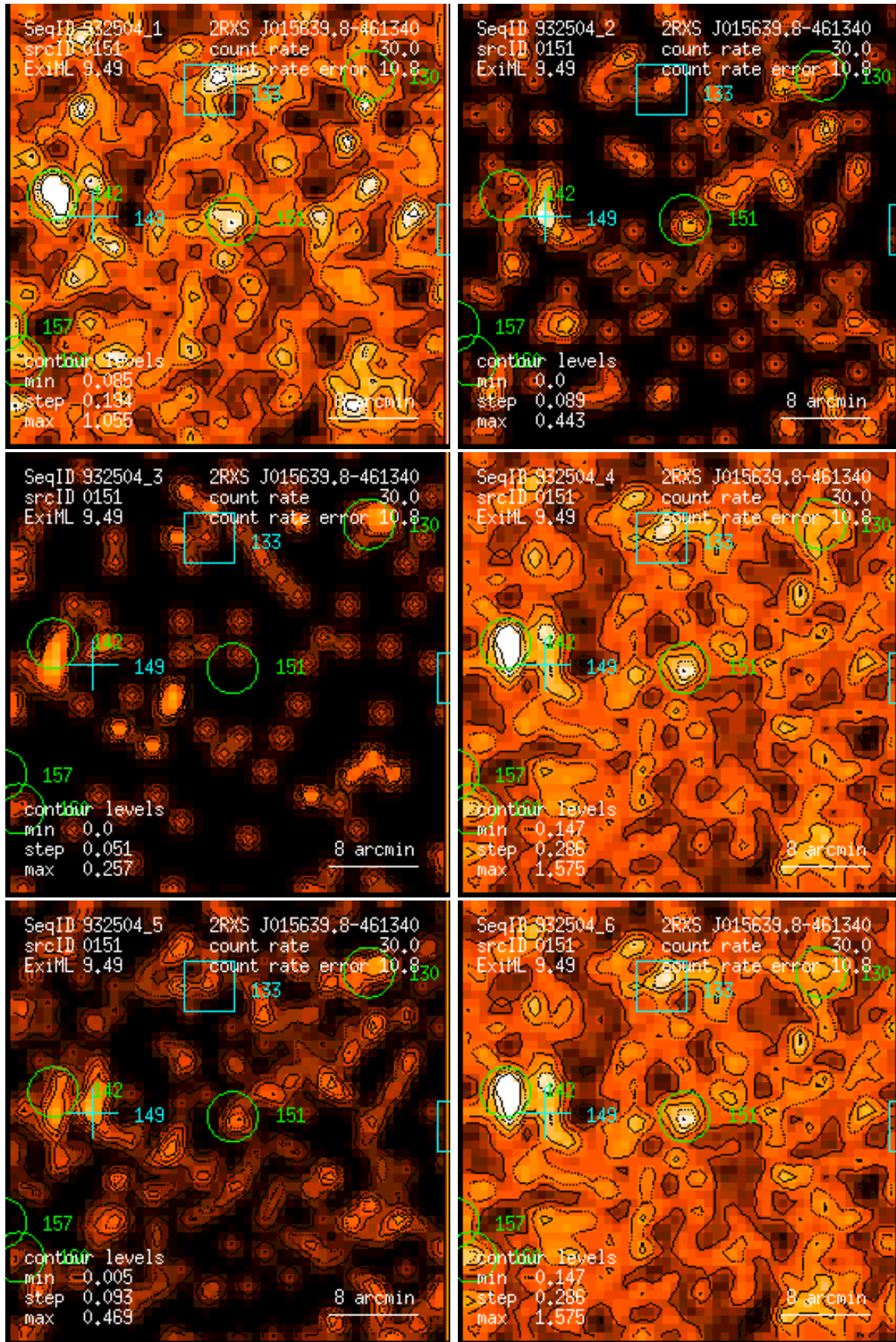
Figure 151: RASS 932504: detection 0151: band rate images, Gaussian filter: (1) PSPC channels 11 – 41, (2) 52 – 90, (3) 91 – 201, (4) 11 – 235, (5) 52 – 201, (6) 11 – 201. Broad band rates in counts/ks. Band rate contour levels in counts/ks/arcmin 2 .
