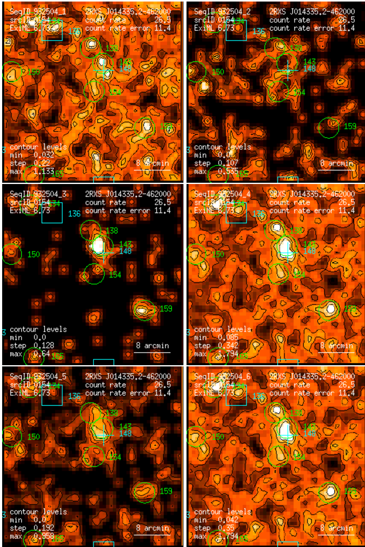
Figure 154: RASS 932504: detection 0154: band rate images, Gaussian filter: (1) PSPC channels 11 – 41, (2) 52 – 90, (3) 91 – 201, (4) 11 – 235, (5) 52 – 201, (6) 11 – 201. Broad band rates in counts/ks. Band rate contour levels in counts/ks/arcmin 2 .
