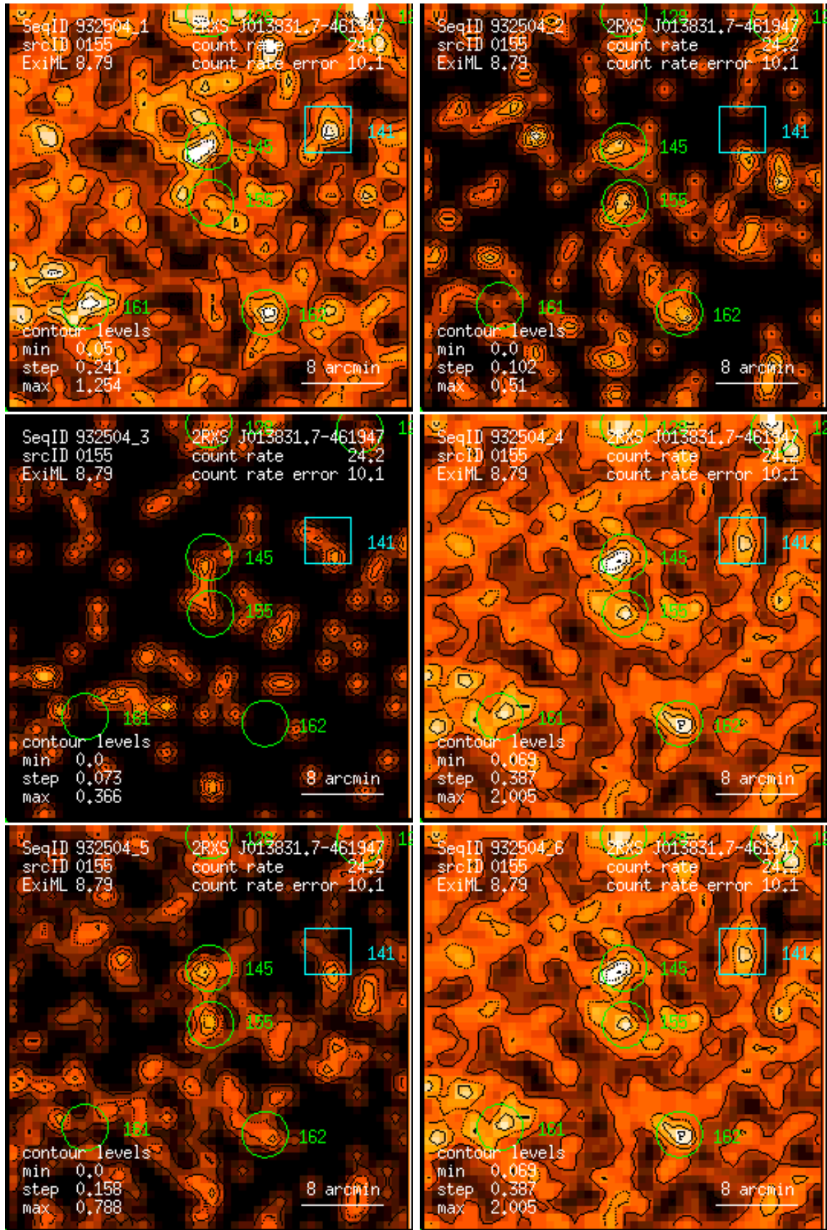
Figure 155: RASS 932504: detection 0155: band rate images, Gaussian filter: (1) PSPC channels 11 – 41, (2) 52 – 90, (3) 91 – 201, (4) 11 – 235, (5) 52 – 201, (6) 11 – 201. Broad band rates in counts/ks. Band rate contour levels in counts/ks/arcmin 2 .
