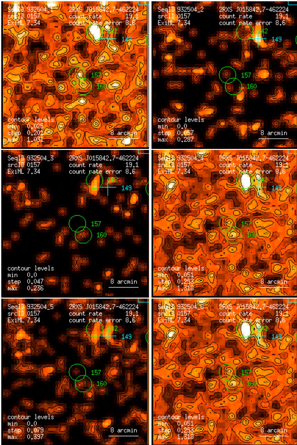
Figure 157: RASS 932504: detection 0157: band rate images, Gaussian filter: (1) PSPC channels 11 – 41, (2) 52 – 90, (3) 91 – 201, (4) 11 – 235, (5) 52 – 201, (6) 11 – 201. Broad band rates in counts/ks. Band rate contour levels in counts/ks/arcmin 2 .
