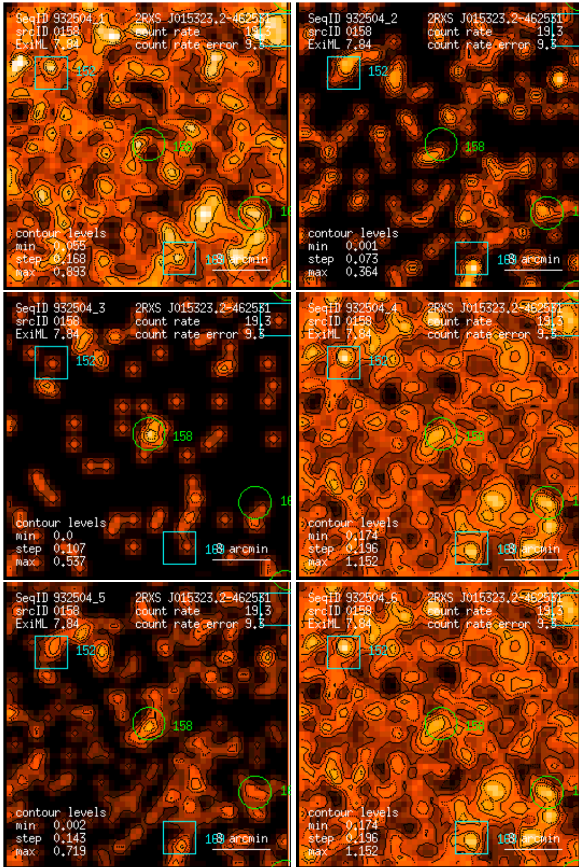
Figure 158: RASS 932504: detection 0158: band rate images, Gaussian filter: (1) PSPC channels 11 – 41, (2) 52 – 90, (3) 91 – 201, (4) 11 – 235, (5) 52 – 201, (6) 11 – 201. Broad band rates in counts/ks. Band rate contour levels in counts/ks/arcmin 2 .
