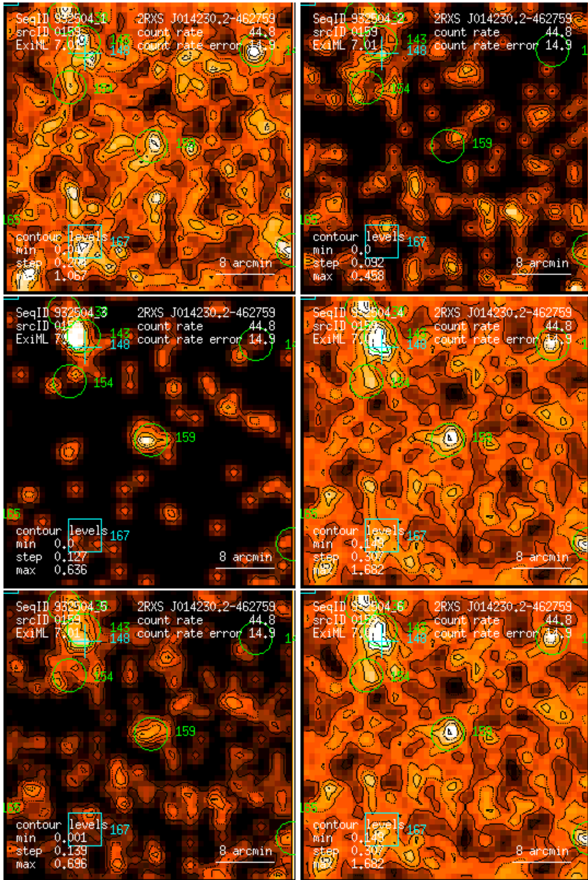
Figure 159: RASS 932504: detection 0159: band rate images, Gaussian filter: (1) PSPC channels 11 – 41, (2) 52 – 90, (3) 91 – 201, (4) 11 – 235, (5) 52 – 201, (6) 11 – 201. Broad band rates in counts/ks. Band rate contour levels in counts/ks/arcmin 2 .
