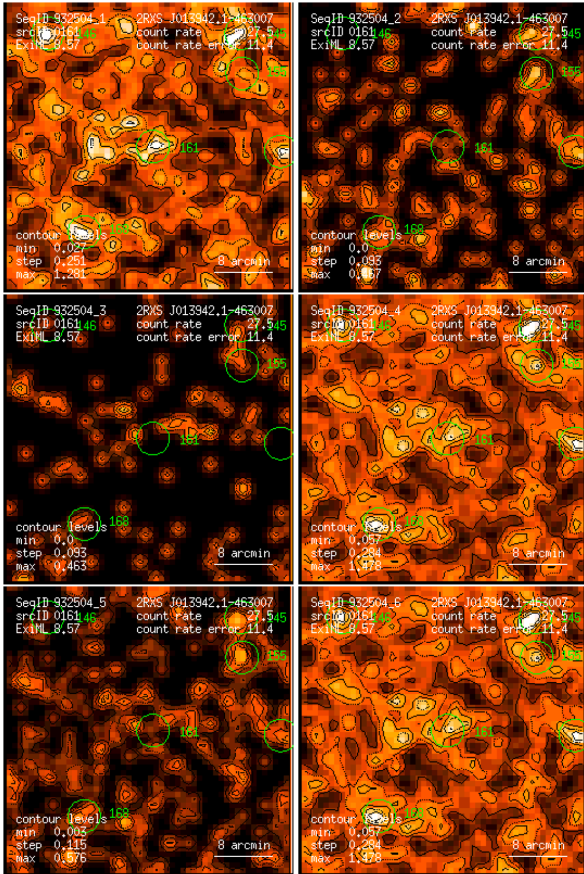
Figure 161: RASS 932504: detection 0161: band rate images, Gaussian filter: (1) PSPC channels 11 – 41, (2) 52 – 90, (3) 91 – 201, (4) 11 – 235, (5) 52 – 201, (6) 11 – 201. Broad band rates in counts/ks. Band rate contour levels in counts/ks/arcmin 2 .
