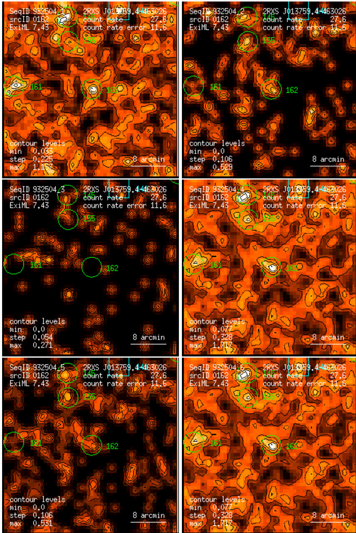
Figure 162: RASS 932504: detection 0162: band rate images, Gaussian filter: (1) PSPC channels 11 – 41, (2) 52 – 90, (3) 91 – 201, (4) 11 – 235, (5) 52 – 201, (6) 11 – 201. Broad band rates in counts/ks. Band rate contour levels in counts/ks/arcmin 2 .
