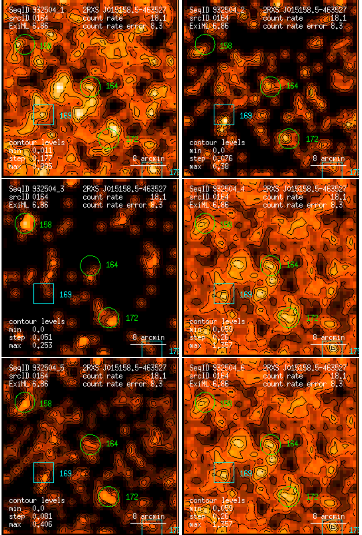
Figure 164: RASS 932504: detection 0164: band rate images, Gaussian filter: (1) PSPC channels 11 – 41, (2) 52 – 90, (3) 91 – 201, (4) 11 – 235, (5) 52 – 201, (6) 11 – 201. Broad band rates in counts/ks. Band rate contour levels in counts/ks/arcmin 2 .
