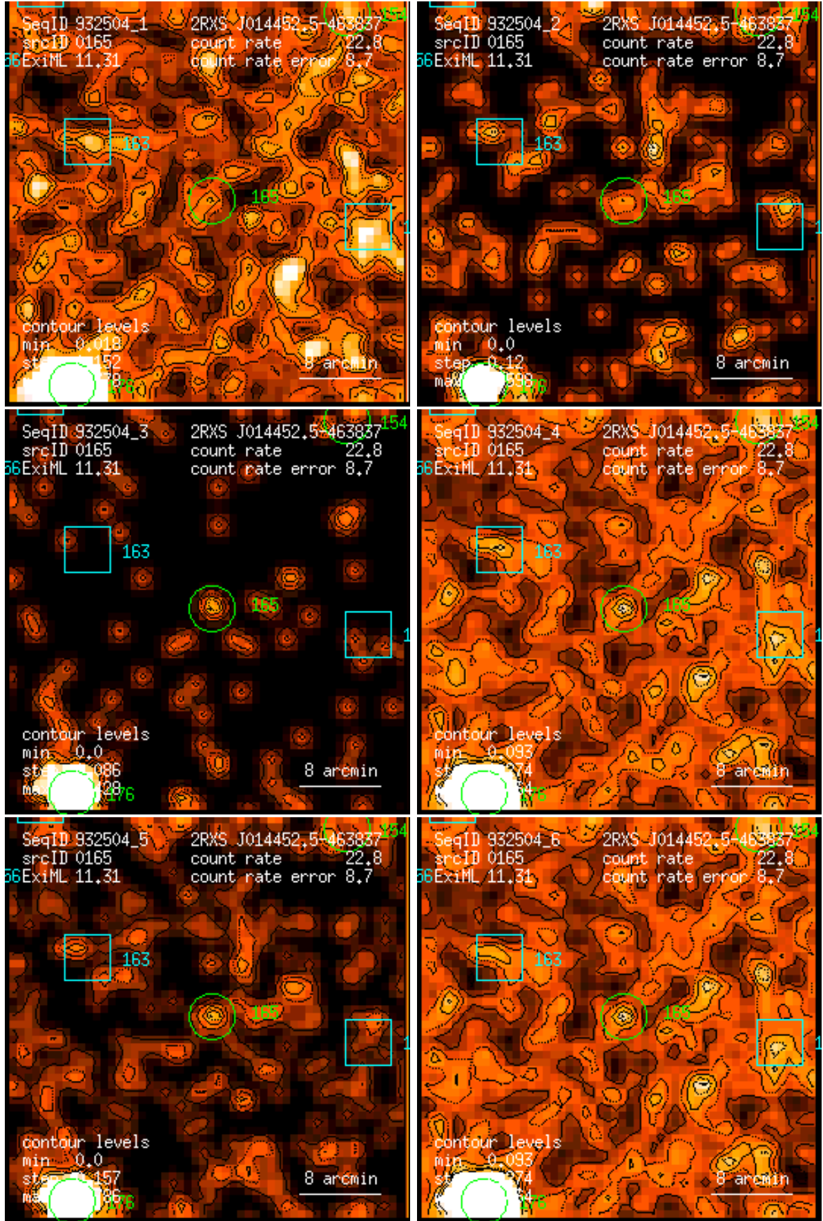
Figure 165: RASS 932504: detection 0165: band rate images, Gaussian filter: (1) PSPC channels 11 – 41, (2) 52 – 90, (3) 91 – 201, (4) 11 – 235, (5) 52 – 201, (6) 11 – 201. Broad band rates in counts/ks. Band rate contour levels in counts/ks/arcmin 2 .
