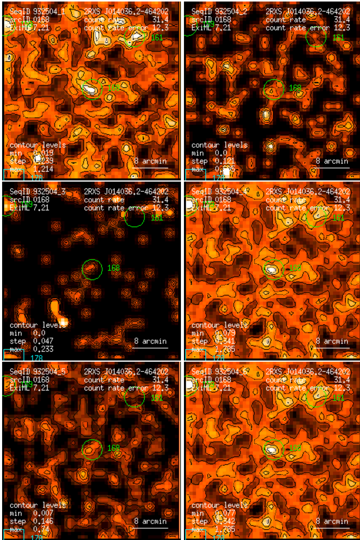
Figure 168: RASS 932504: detection 0168: band rate images, Gaussian filter: (1) PSPC channels 11 – 41, (2) 52 – 90, (3) 91 – 201, (4) 11 – 235, (5) 52 – 201, (6) 11 – 201. Broad band rates in counts/ks. Band rate contour levels in counts/ks/arcmin 2 .
