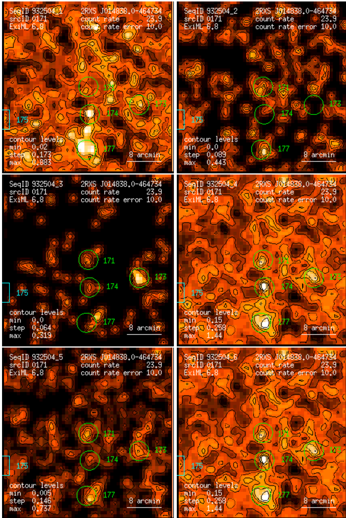
Figure 171: RASS 932504: detection 0171: band rate images, Gaussian filter: (1) PSPC channels 11 – 41, (2) 52 – 90, (3) 91 – 201, (4) 11 – 235, (5) 52 – 201, (6) 11 – 201. Broad band rates in counts/ks. Band rate contour levels in counts/ks/arcmin 2 .
