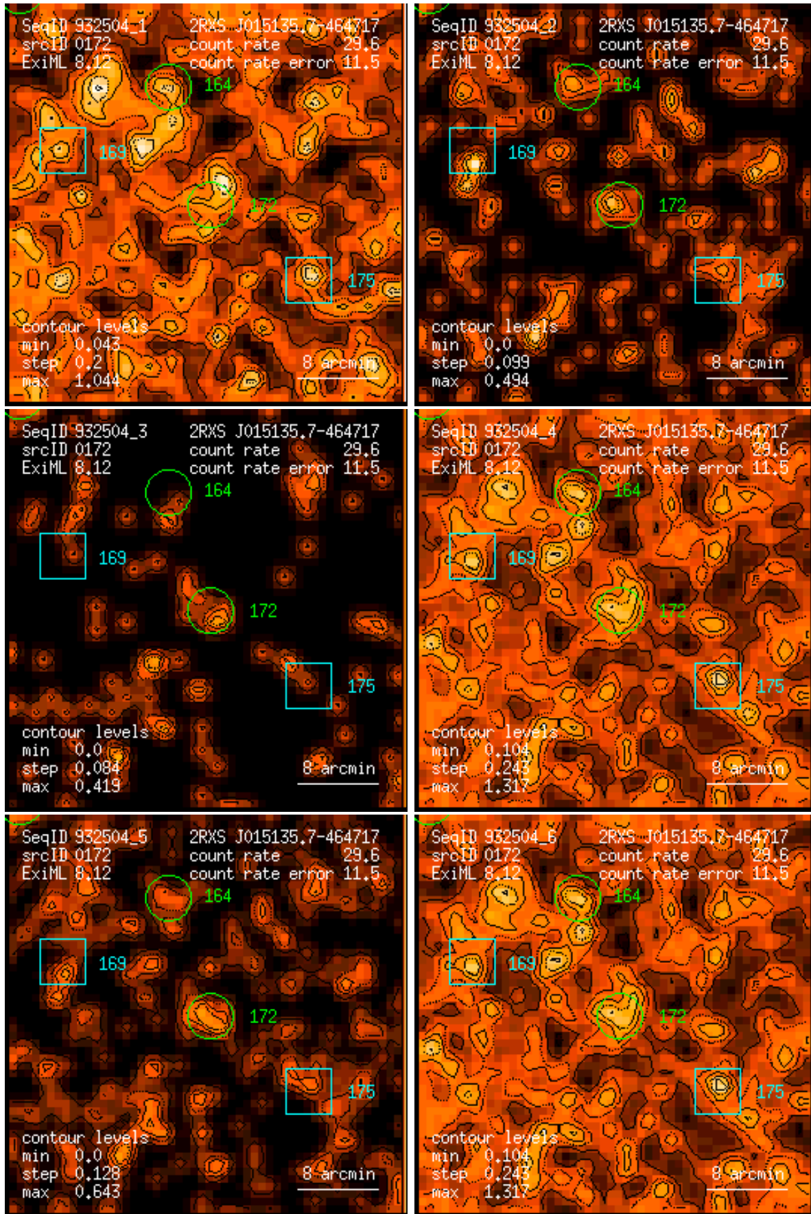
Figure 172: RASS 932504: detection 0172: band rate images, Gaussian filter: (1) PSPC channels 11 – 41, (2) 52 – 90, (3) 91 – 201, (4) 11 – 235, (5) 52 – 201, (6) 11 – 201. Broad band rates in counts/ks. Band rate contour levels in counts/ks/arcmin 2 .
