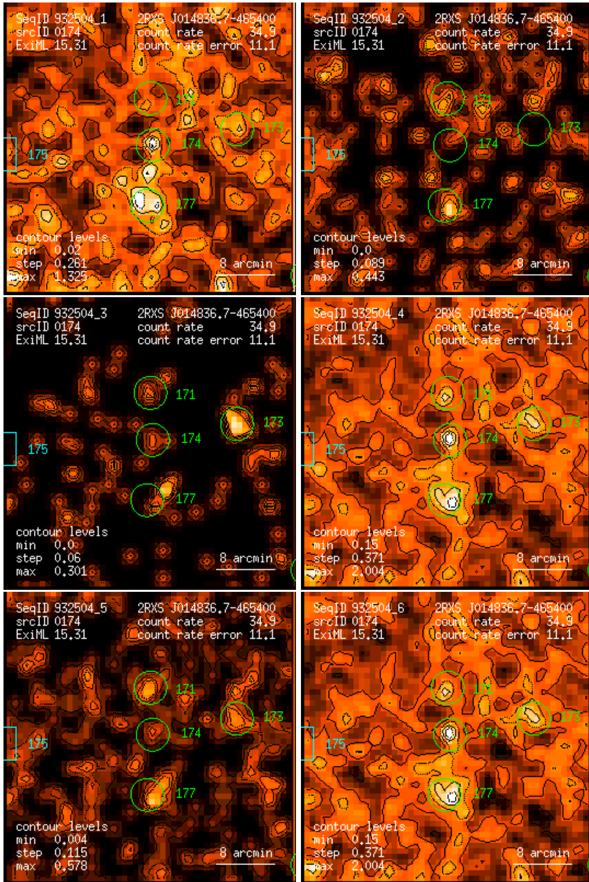
Figure 174: RASS 932504: detection 0174: band rate images, Gaussian filter: (1) PSPC channels 11 – 41, (2) 52 – 90, (3) 91 – 201, (4) 11 – 235, (5) 52 – 201, (6) 11 – 201. Broad band rates in counts/ks. Band rate contour levels in counts/ks/arcmin 2 .
