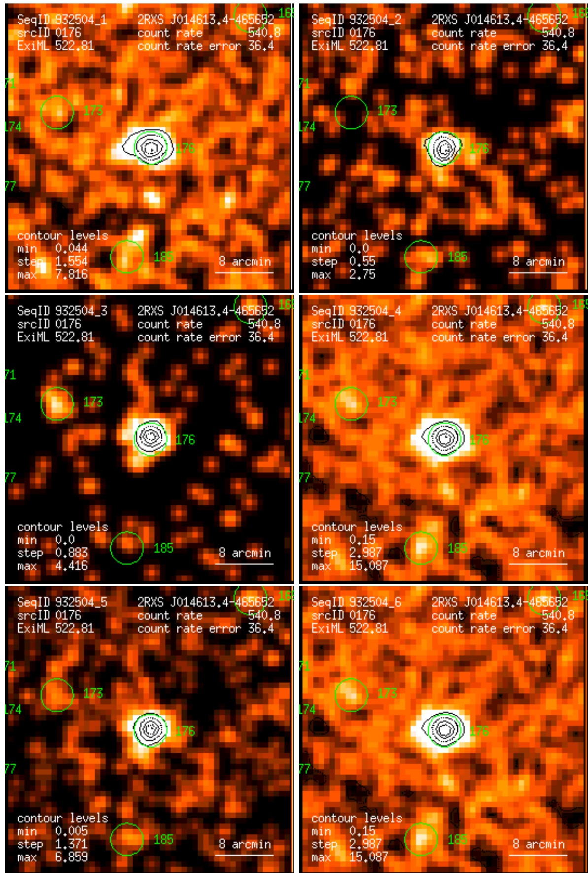
Figure 176: RASS 932504: detection 0176: band rate images, Gaussian filter: (1) PSPC channels 11 – 41, (2) 52 – 90, (3) 91 – 201, (4) 11 – 235, (5) 52 – 201, (6) 11 – 201. Broad band rates in counts/ks. Band rate contour levels in counts/ks/arcmin 2 .
