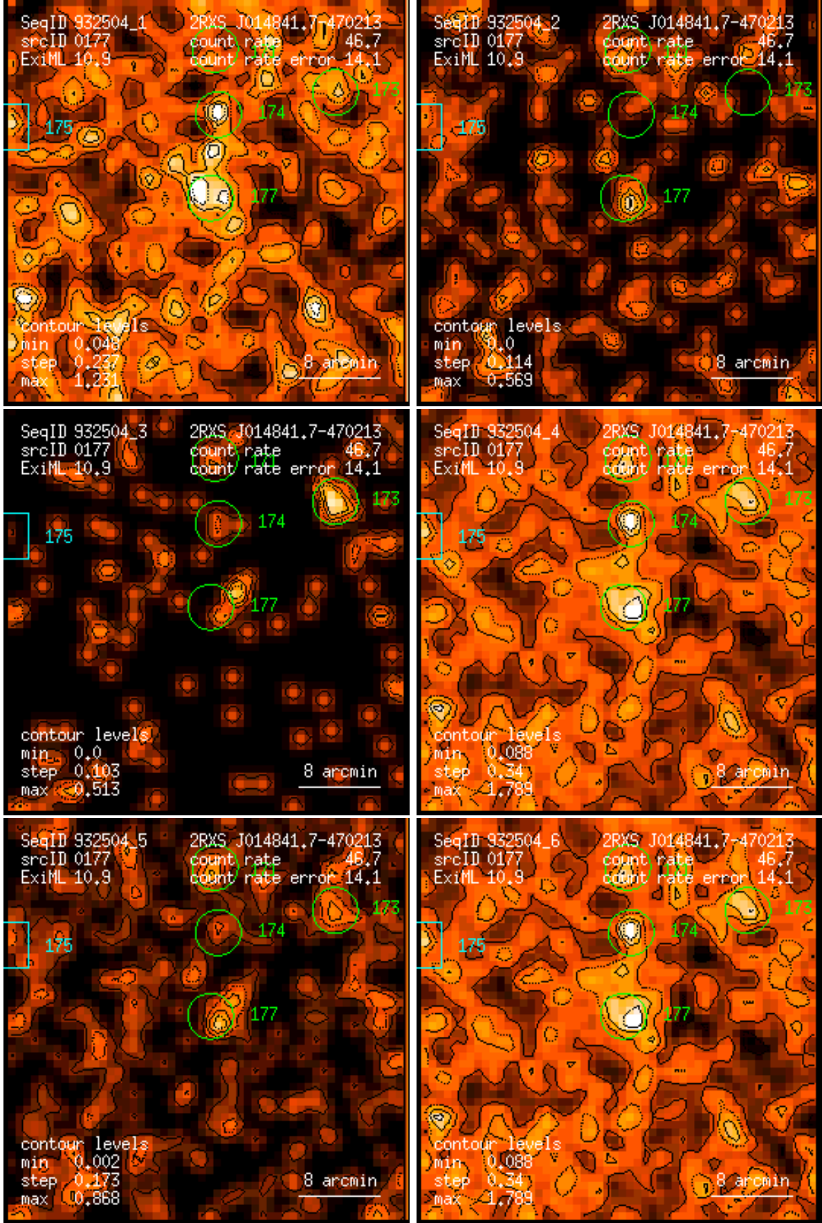
Figure 177: RASS 932504: detection 0177: band rate images, Gaussian filter: (1) PSPC channels 11 – 41, (2) 52 – 90, (3) 91 – 201, (4) 11 – 235, (5) 52 – 201, (6) 11 – 201. Broad band rates in counts/ks. Band rate contour levels in counts/ks/arcmin 2 .
