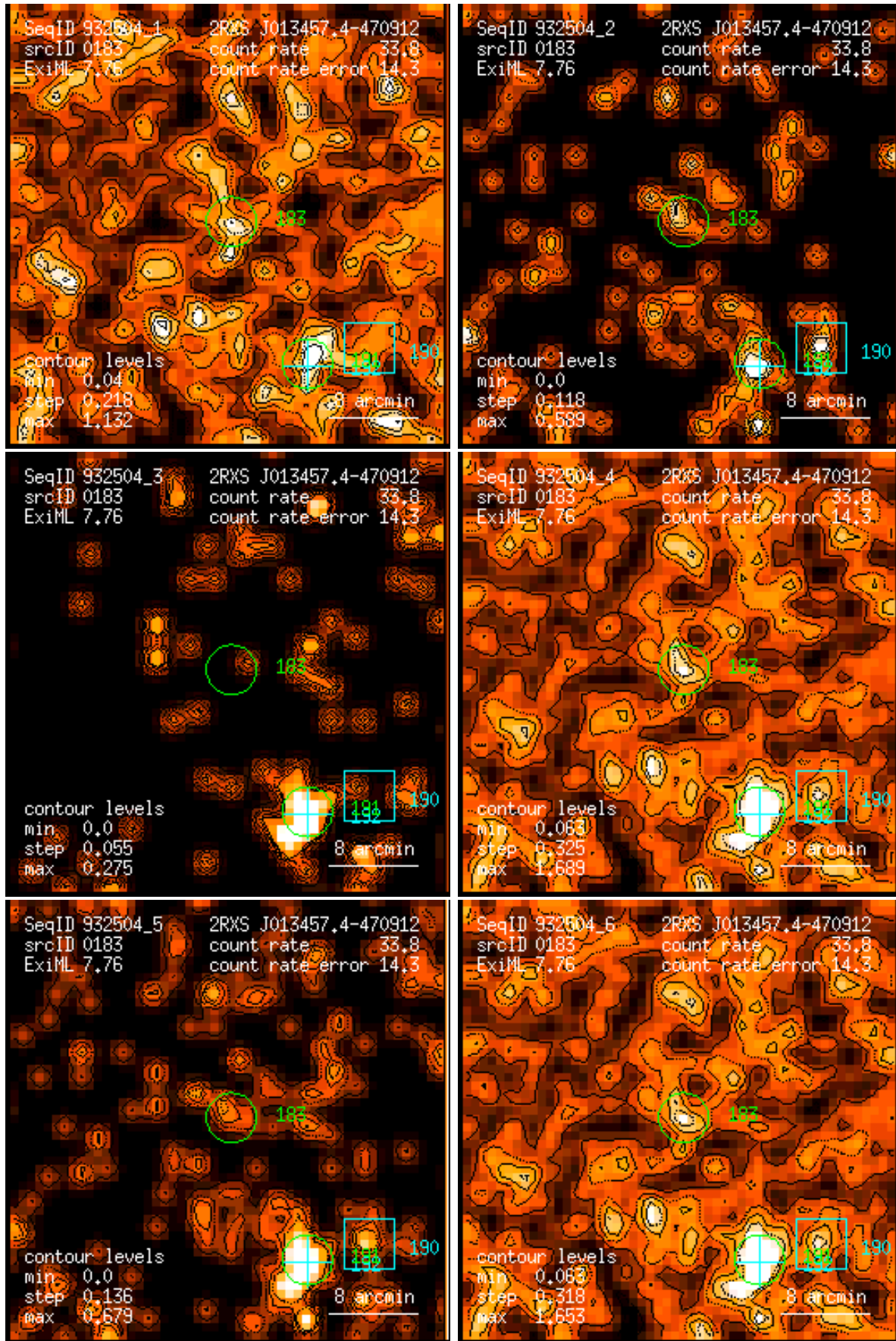
Figure 183: RASS 932504: detection 0183: band rate images, Gaussian filter: (1) PSPC channels 11 – 41, (2) 52 – 90, (3) 91 – 201, (4) 11 – 235, (5) 52 – 201, (6) 11 – 201. Broad band rates in counts/ks. Band rate contour levels in counts/ks/arcmin 2 .
