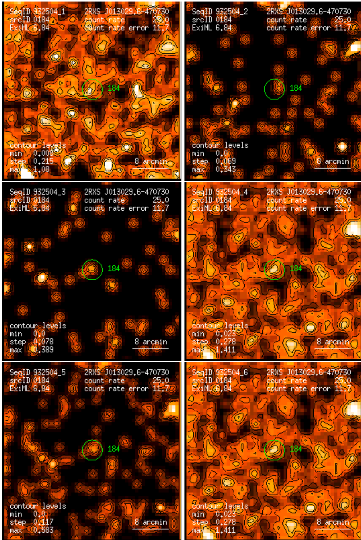
Figure 184: RASS 932504: detection 0184: band rate images, Gaussian filter: (1) PSPC channels 11 – 41, (2) 52 – 90, (3) 91 – 201, (4) 11 – 235, (5) 52 – 201, (6) 11 – 201. Broad band rates in counts/ks. Band rate contour levels in counts/ks/arcmin 2 .
