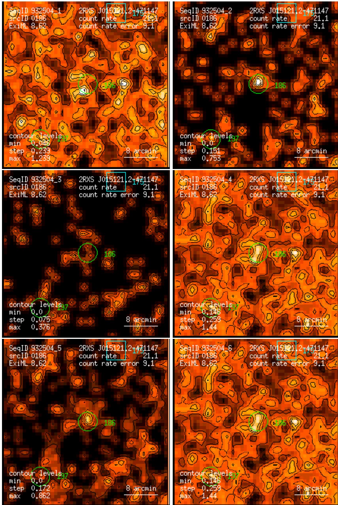
Figure 186: RASS 932504: detection 0186: band rate images, Gaussian filter: (1) PSPC channels 11 – 41, (2) 52 – 90, (3) 91 – 201, (4) 11 – 235, (5) 52 – 201, (6) 11 – 201. Broad band rates in counts/ks. Band rate contour levels in counts/ks/arcmin 2 .
