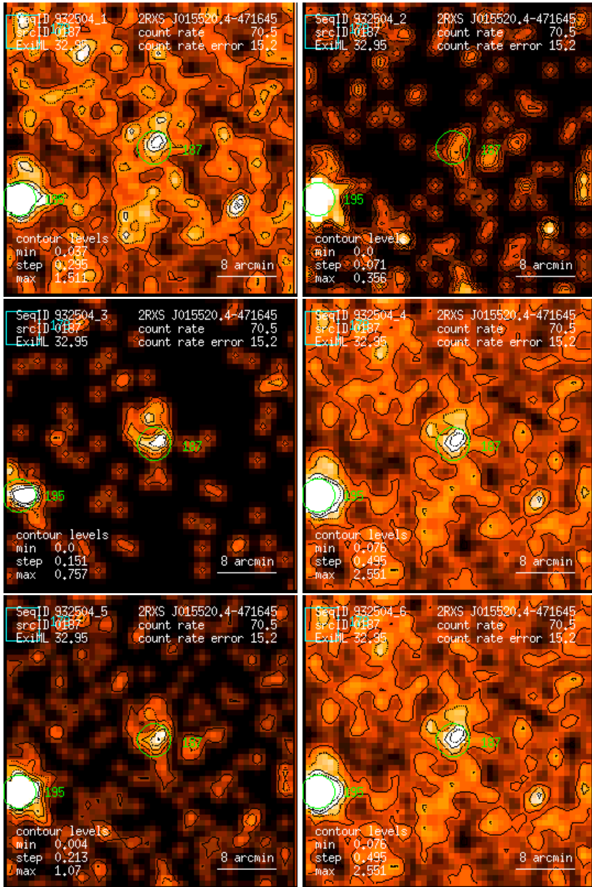
Figure 187: RASS 932504: detection 0187: band rate images, Gaussian filter: (1) PSPC channels 11 – 41, (2) 52 – 90, (3) 91 – 201, (4) 11 – 235, (5) 52 – 201, (6) 11 – 201. Broad band rates in counts/ks. Band rate contour levels in counts/ks/arcmin 2 .
