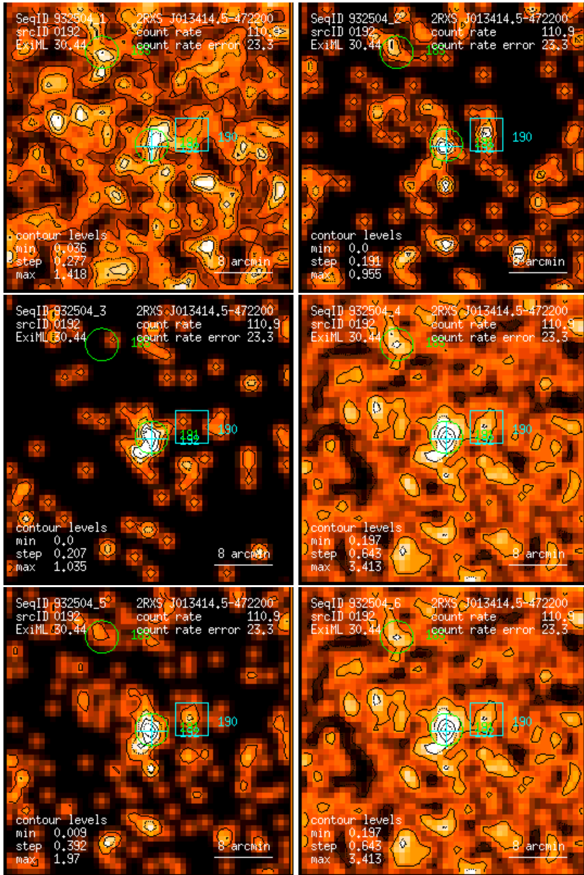
Figure 192: RASS 932504: detection 0192: band rate images, Gaussian filter: (1) PSPC channels 11 – 41, (2) 52 – 90, (3) 91 – 201, (4) 11 – 235, (5) 52 – 201, (6) 11 – 201. Broad band rates in counts/ks. Band rate contour levels in counts/ks/arcmin 2 .
