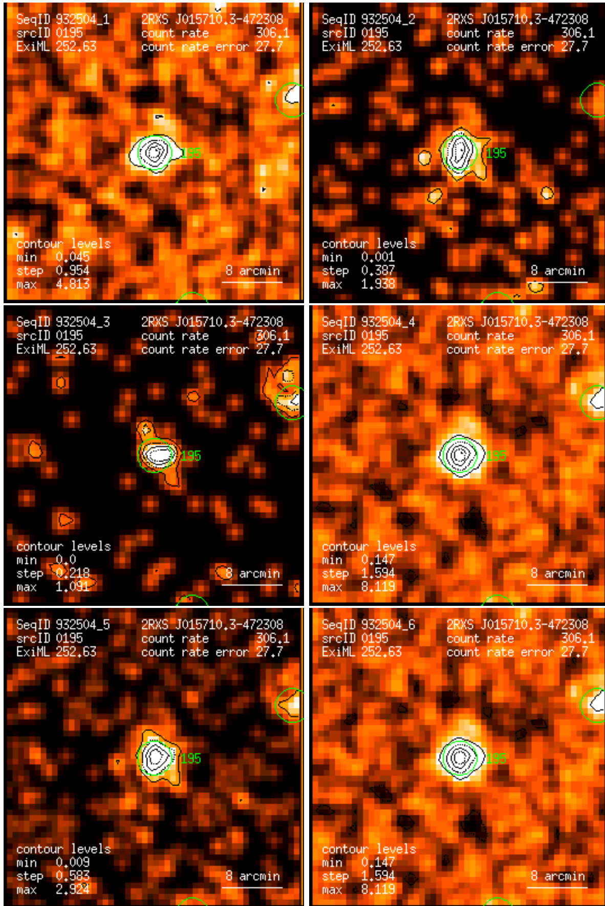
Figure 195: RASS 932504: detection 0195: band rate images, Gaussian filter: (1) PSPC channels 11 – 41, (2) 52 – 90, (3) 91 – 201, (4) 11 – 235, (5) 52 – 201, (6) 11 – 201. Broad band rates in counts/ks. Band rate contour levels in counts/ks/arcmin 2 .
