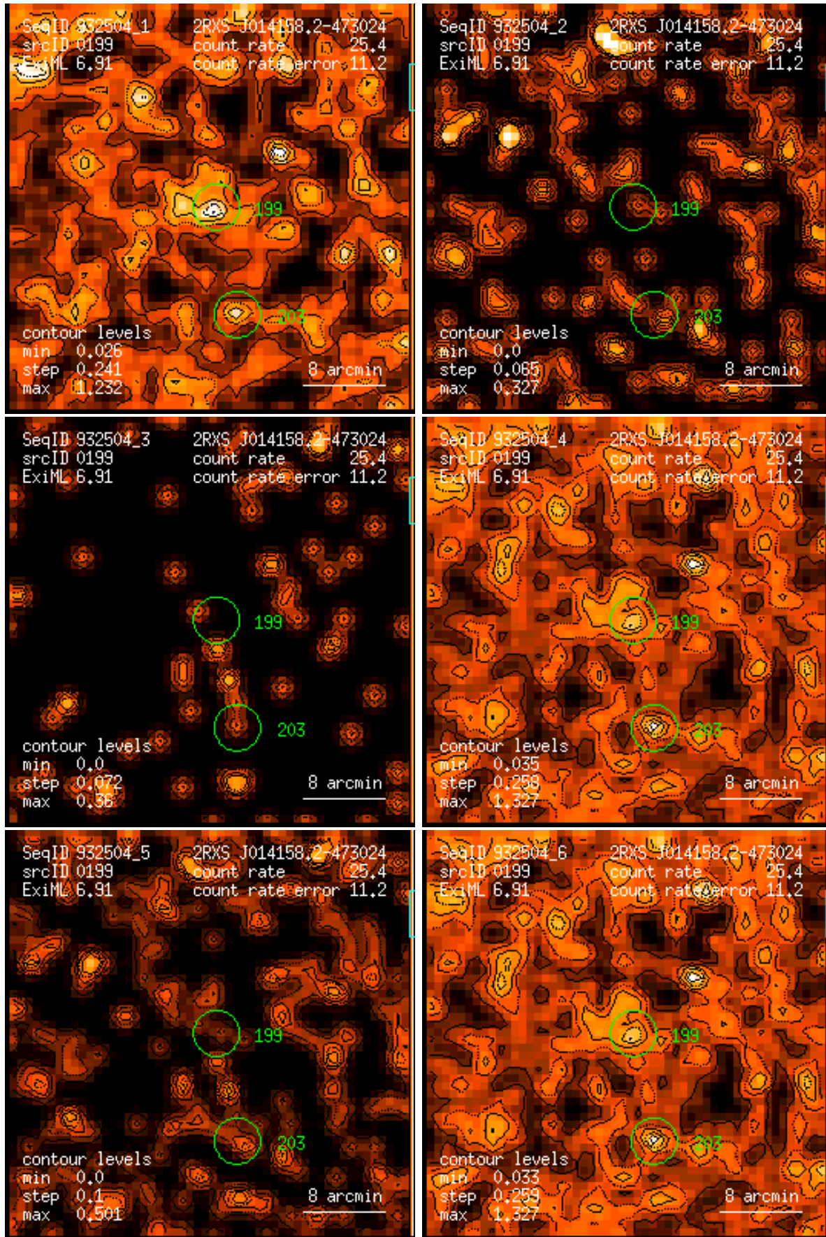
Figure 199: RASS 932504: detection 0199: band rate images, Gaussian filter: (1) PSPC channels 11 – 41, (2) 52 – 90, (3) 91 – 201, (4) 11 – 235, (5) 52 – 201, (6) 11 – 201. Broad band rates in counts/ks. Band rate contour levels in counts/ks/arcmin 2 .
