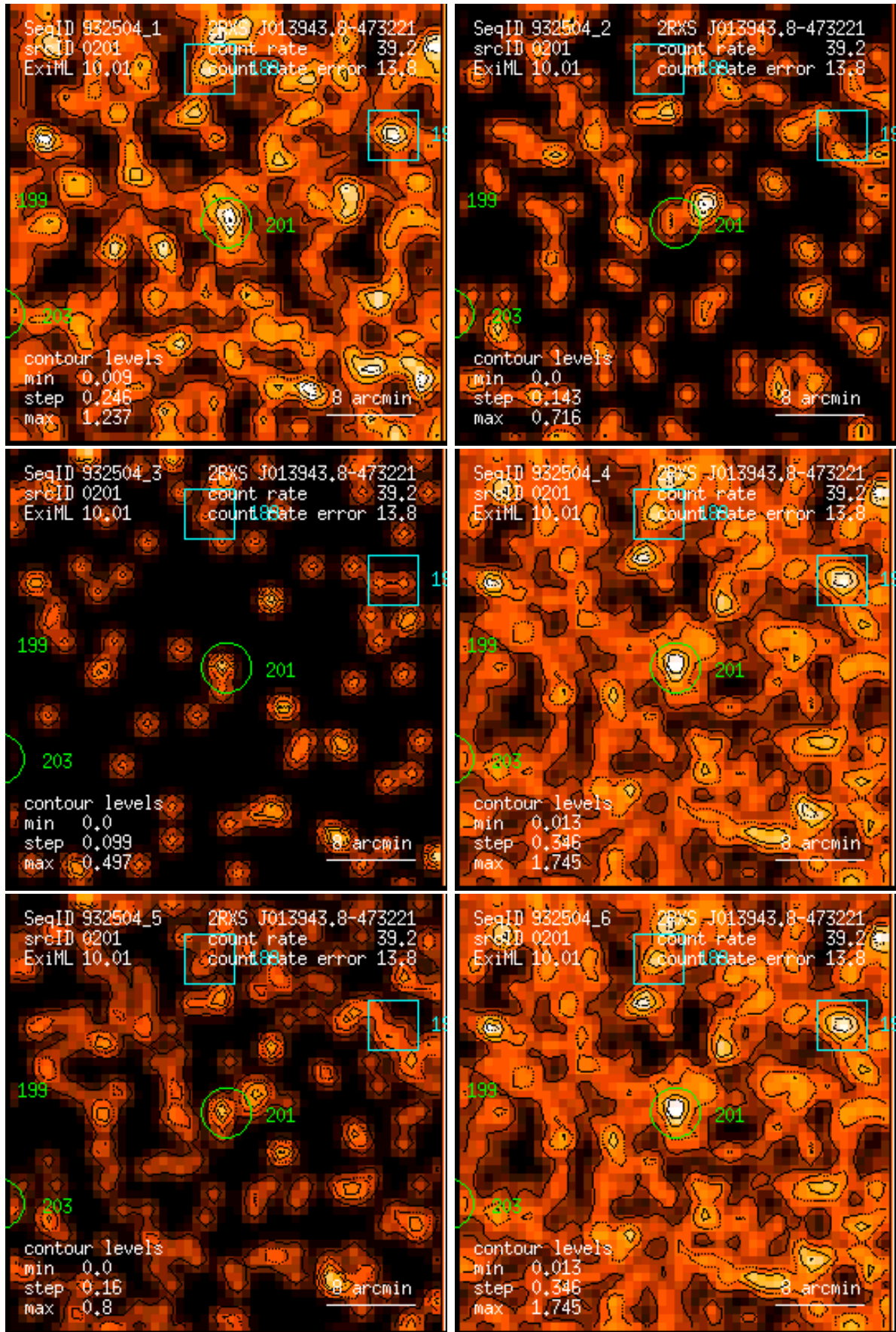
Figure 201: RASS 932504: detection 0201: band rate images, Gaussian filter: (1) PSPC channels 11 – 41, (2) 52 – 90, (3) 91 – 201, (4) 11 – 235, (5) 52 – 201, (6) 11 – 201. Broad band rates in counts/ks. Band rate contour levels in counts/ks/arcmin 2 .
