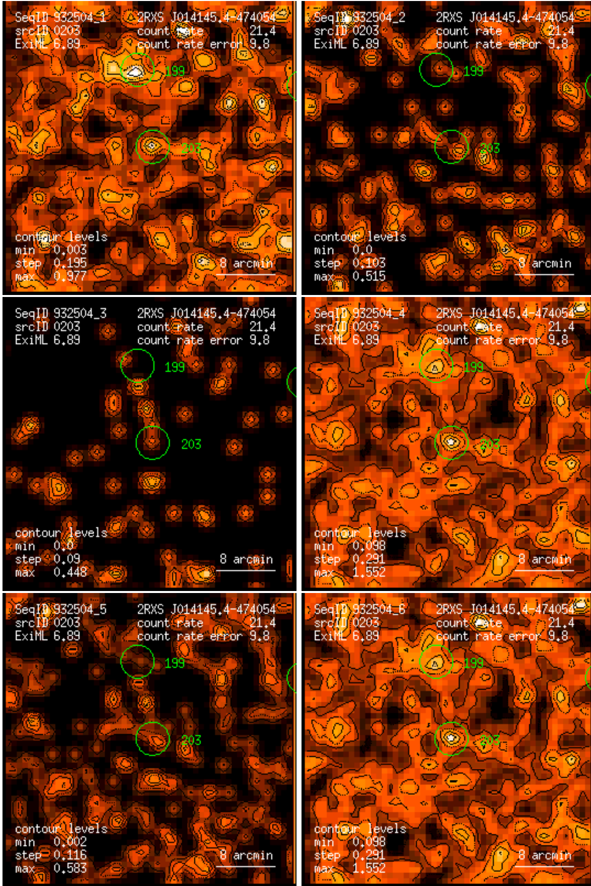
Figure 203: RASS 932504: detection 0203: band rate images, Gaussian filter: (1) PSPC channels 11 – 41, (2) 52 – 90, (3) 91 – 201, (4) 11 – 235, (5) 52 – 201, (6) 11 – 201. Broad band rates in counts/ks. Band rate contour levels in counts/ks/arcmin 2 .
