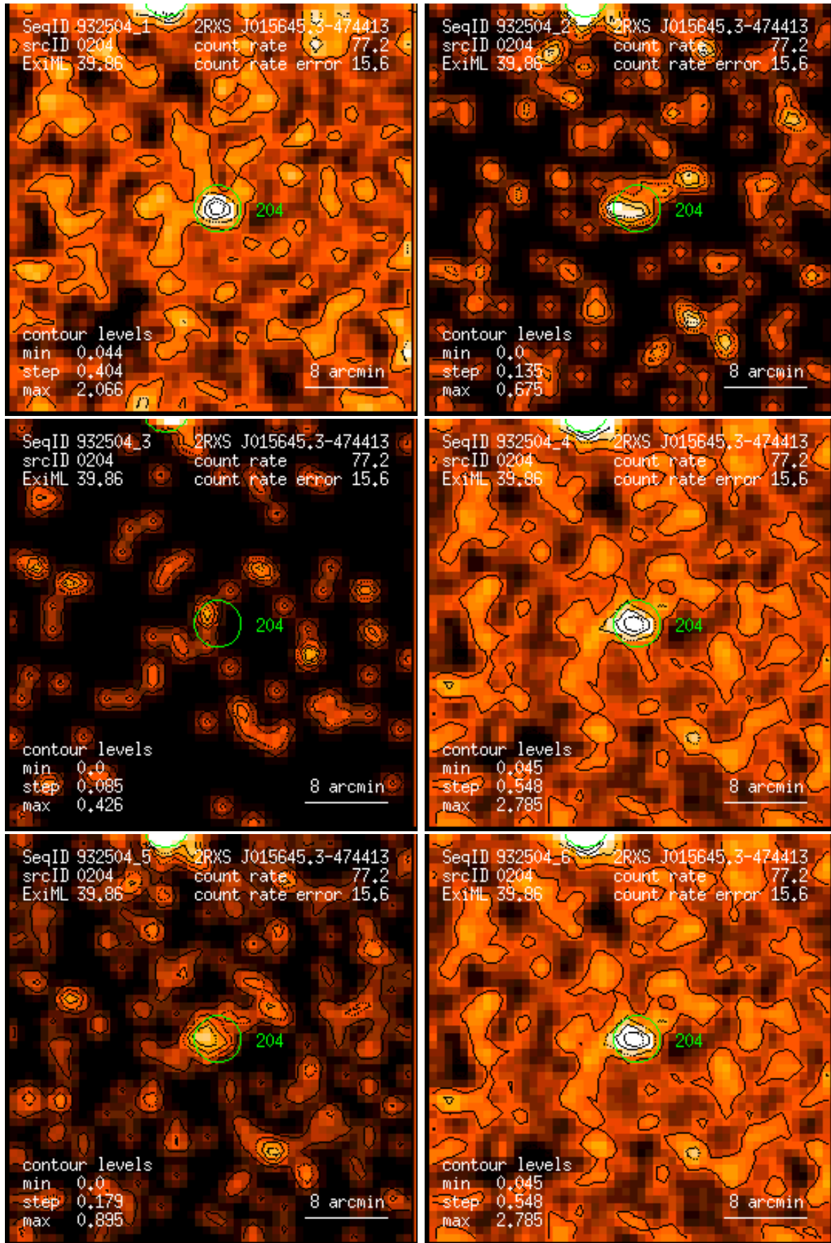
Figure 204: RASS 932504: detection 0204: band rate images, Gaussian filter: (1) PSPC channels 11 – 41, (2) 52 – 90, (3) 91 – 201, (4) 11 – 235, (5) 52 – 201, (6) 11 – 201. Broad band rates in counts/ks. Band rate contour levels in counts/ks/arcmin 2 .
