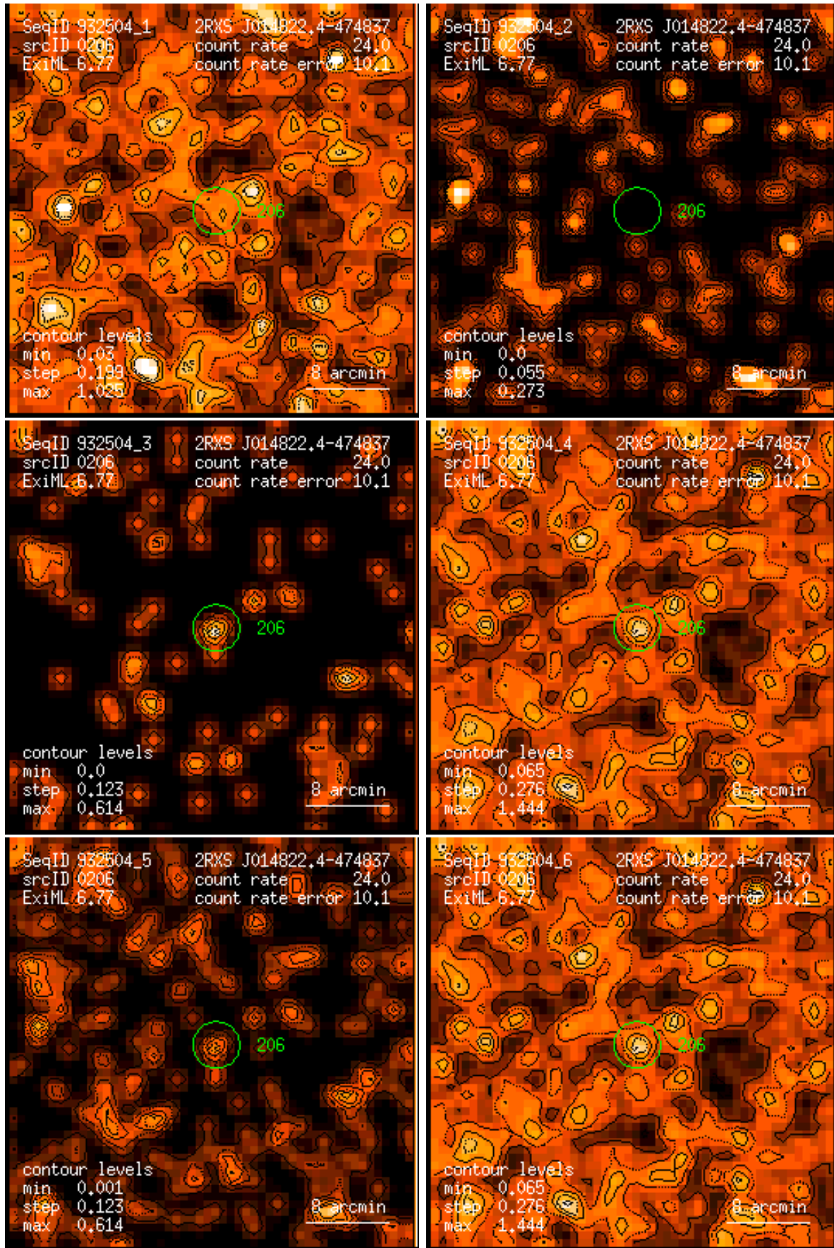
Figure 206: RASS 932504: detection 0206: band rate images, Gaussian filter: (1) PSPC channels 11 – 41, (2) 52 – 90, (3) 91 – 201, (4) 11 – 235, (5) 52 – 201, (6) 11 – 201. Broad band rates in counts/ks. Band rate contour levels in counts/ks/arcmin 2 .
