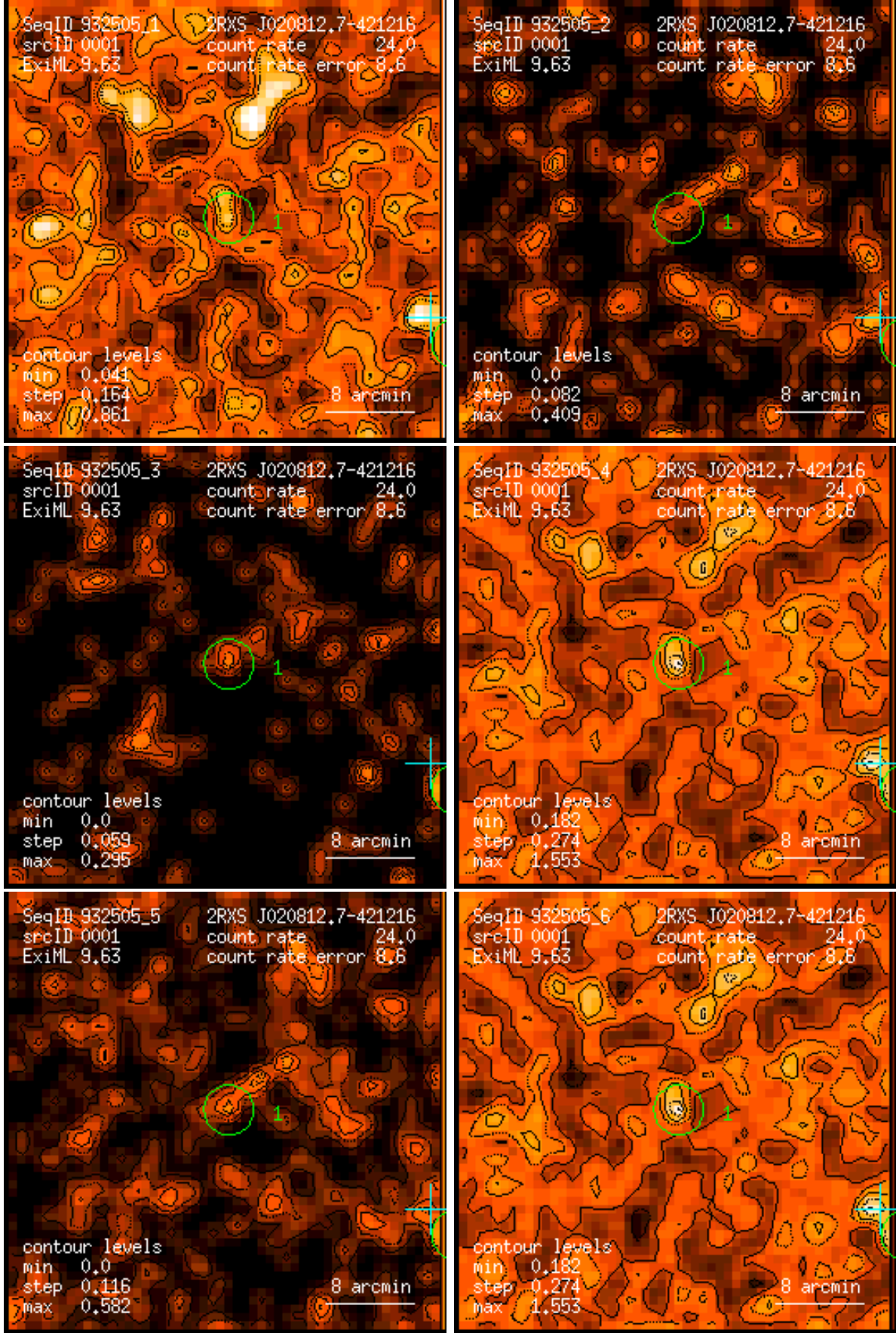
Figure 1: RASS 932505: detection 0001: band rate images, Gaussian filter: (1) PSPC channels 11 – 41, (2) 52 – 90, (3) 91 – 201, (4) 11 – 235, (5) 52 – 201, (6) 11 – 201. Broad band rates in counts/ks. Band rate contour levels in counts/ks/arcmin 2 .
