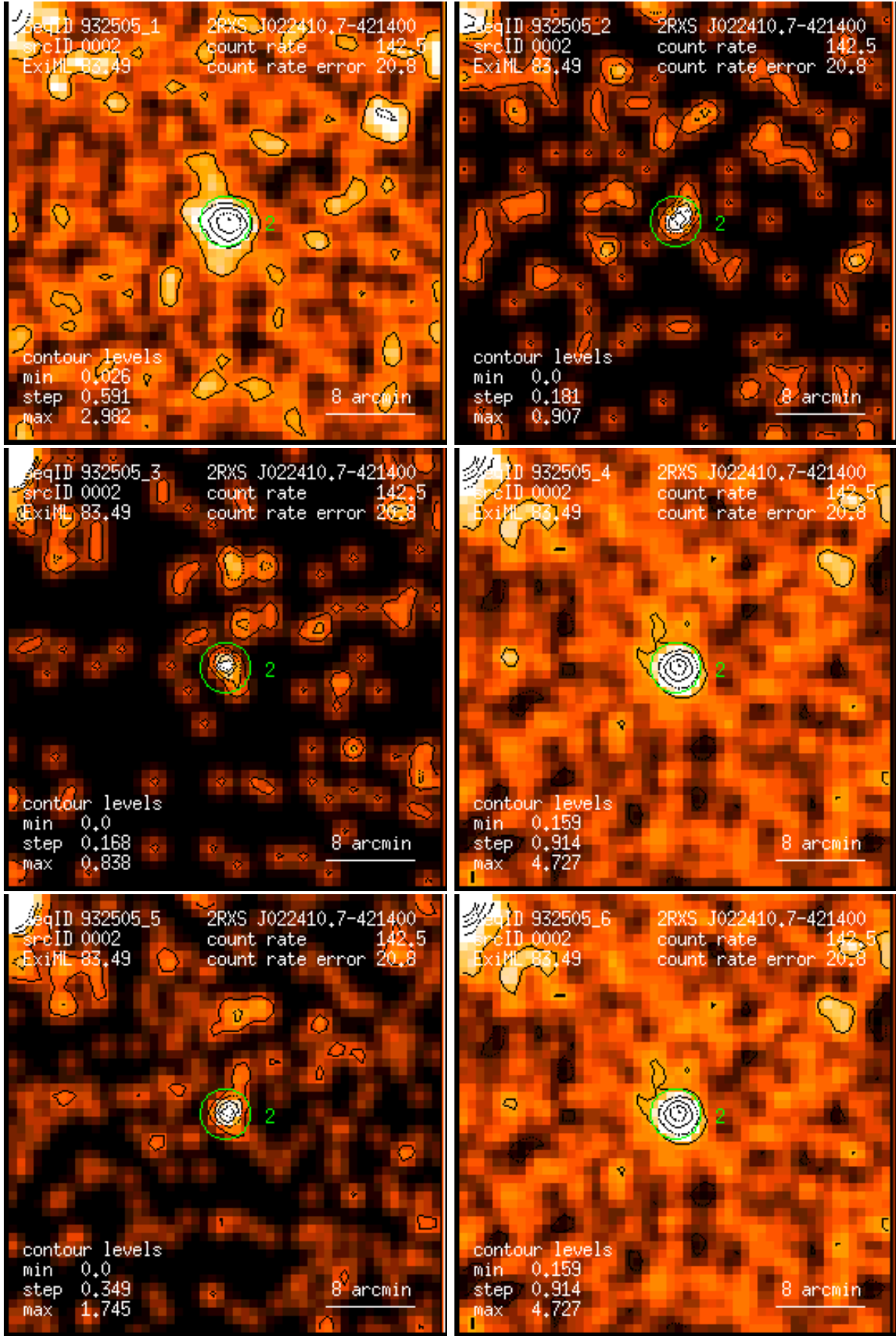
Figure 2: RASS 932505: detection 0002: band rate images, Gaussian filter: (1) PSPC channels 11 – 41, (2) 52 – 90, (3) 91 – 201, (4) 11 – 235, (5) 52 – 201, (6) 11 – 201. Broad band rates in counts/ks. Band rate contour levels in counts/ks/arcmin 2 .
