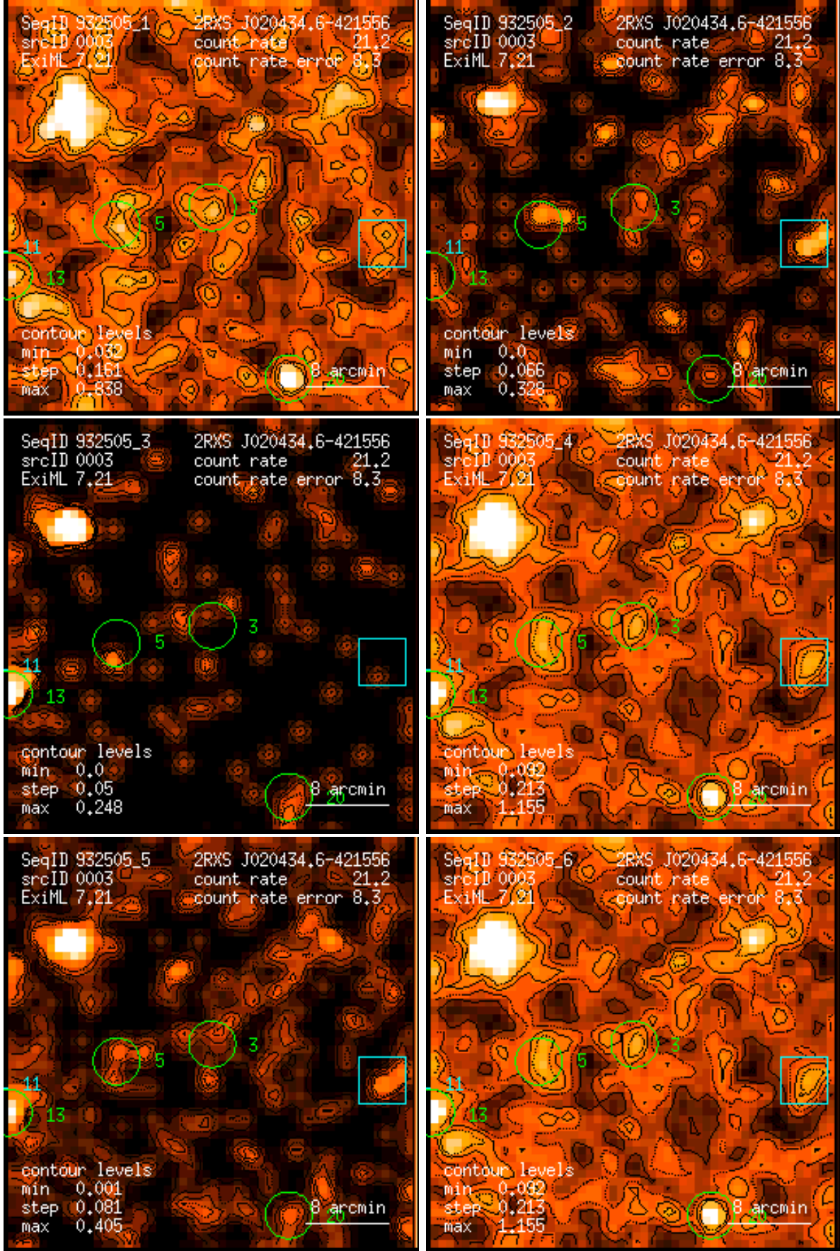
Figure 3: RASS 932505: detection 0003: band rate images, Gaussian filter: (1) PSPC channels 11 – 41, (2) 52 – 90, (3) 91 – 201, (4) 11 – 235, (5) 52 – 201, (6) 11 – 201. Broad band rates in counts/ks. Band rate contour levels in counts/ks/arcmin 2 .
