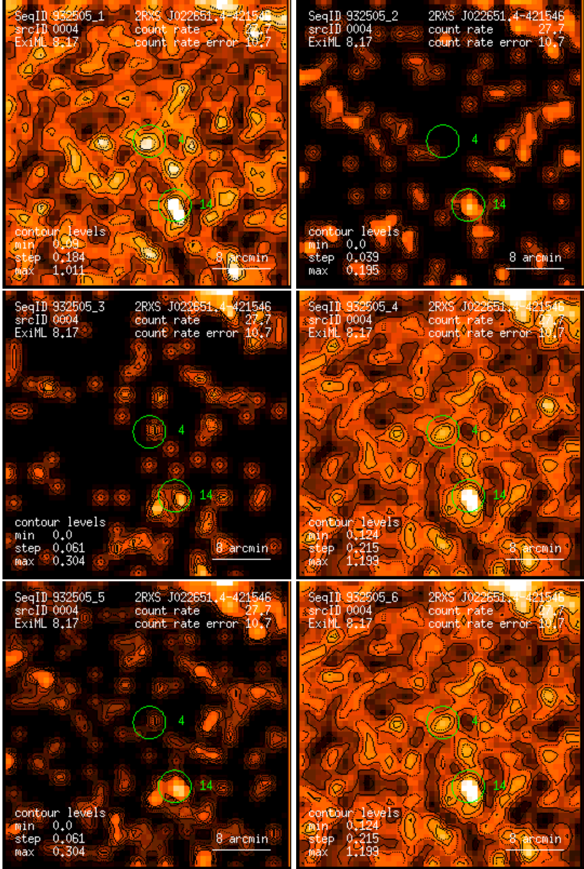
Figure 4: RASS 932505: detection 0004: band rate images, Gaussian filter: (1) PSPC channels 11 – 41, (2) 52 – 90, (3) 91 – 201, (4) 11 – 235, (5) 52 – 201, (6) 11 – 201. Broad band rates in counts/ks. Band rate contour levels in counts/ks/arcmin 2 .
