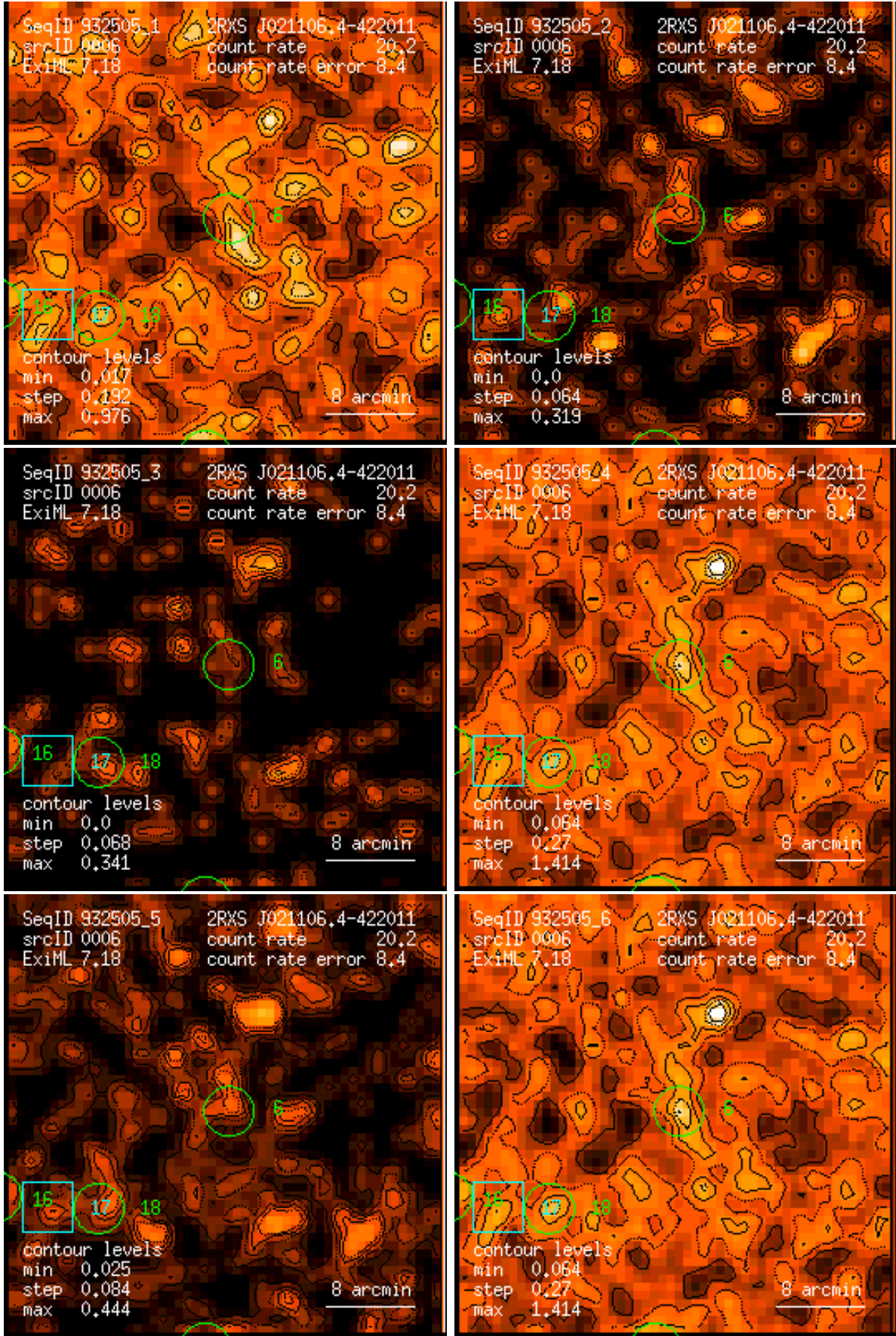
Figure 6: RASS 932505: detection 0006: band rate images, Gaussian filter: (1) PSPC channels 11 – 41, (2) 52 – 90, (3) 91 – 201, (4) 11 – 235, (5) 52 – 201, (6) 11 – 201. Broad band rates in counts/ks. Band rate contour levels in counts/ks/arcmin 2 .
