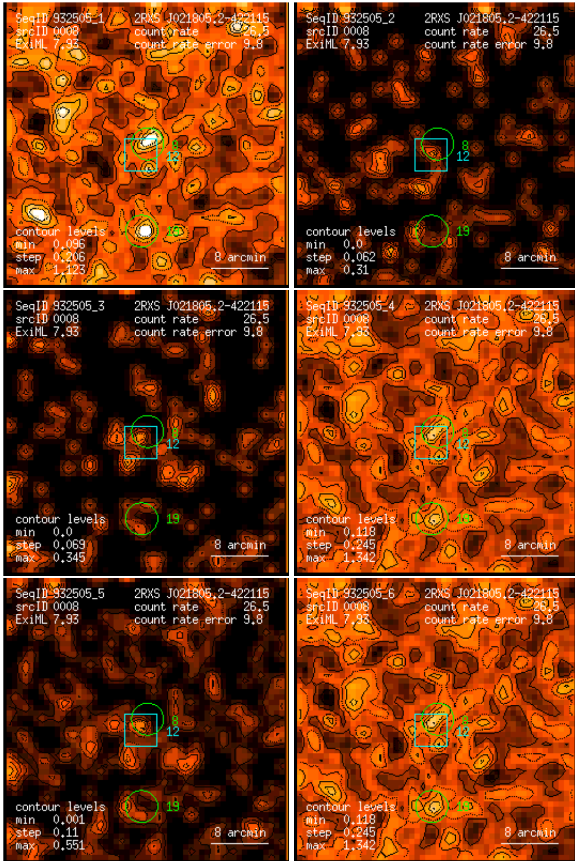
Figure 8: RASS 932505: detection 0008: band rate images, Gaussian filter: (1) PSPC channels 11 – 41, (2) 52 – 90, (3) 91 – 201, (4) 11 – 235, (5) 52 – 201, (6) 11 – 201. Broad band rates in counts/ks. Band rate contour levels in counts/ks/arcmin 2 .
