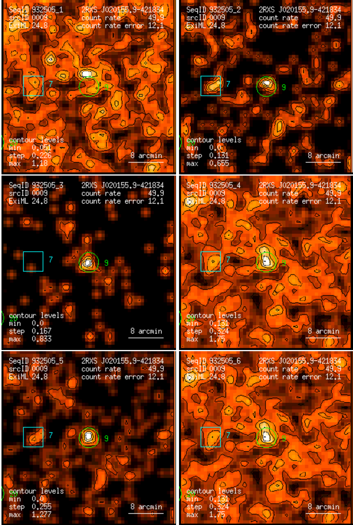
Figure 9: RASS 932505: detection 0009: band rate images, Gaussian filter: (1) PSPC channels 11 – 41, (2) 52 – 90, (3) 91 – 201, (4) 11 – 235, (5) 52 – 201, (6) 11 – 201. Broad band rates in counts/ks. Band rate contour levels in counts/ks/arcmin 2 .
