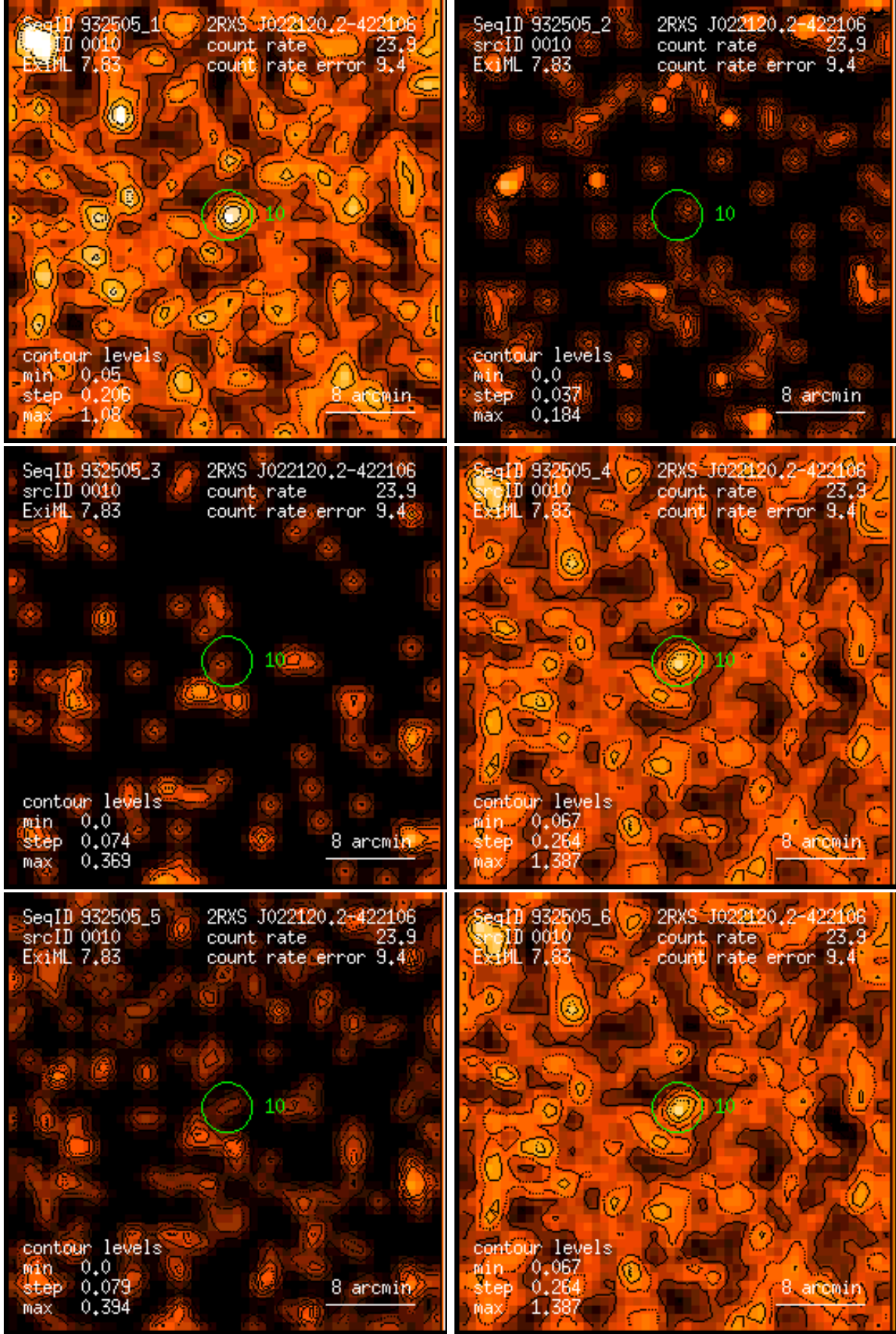
Figure 10: RASS 932505: detection 0010: band rate images, Gaussian filter: (1) PSPC channels 11 – 41, (2) 52 – 90, (3) 91 – 201, (4) 11 – 235, (5) 52 – 201, (6) 11 – 201. Broad band rates in counts/ks. Band rate contour levels in counts/ks/arcmin 2 .
