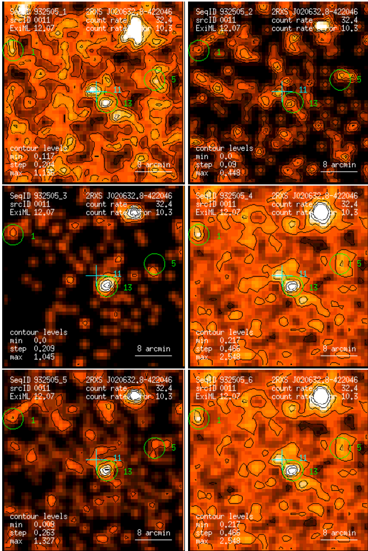
Figure 11: RASS 932505: detection 0011: band rate images, Gaussian filter: (1) PSPC channels 11 – 41, (2) 52 – 90, (3) 91 – 201, (4) 11 – 235, (5) 52 – 201, (6) 11 – 201. Broad band rates in counts/ks. Band rate contour levels in counts/ks/arcmin 2 .
