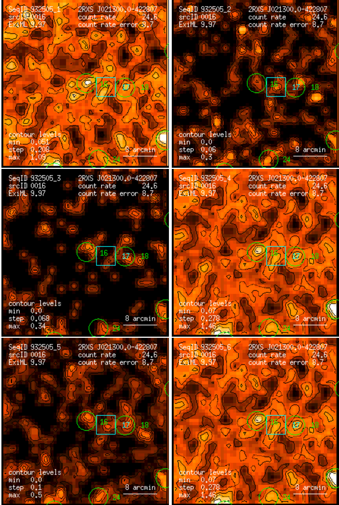
Figure 16: RASS 932505: detection 0016: band rate images, Gaussian filter: (1) PSPC channels 11 – 41, (2) 52 – 90, (3) 91 – 201, (4) 11 – 235, (5) 52 – 201, (6) 11 – 201. Broad band rates in counts/ks. Band rate contour levels in counts/ks/arcmin 2 .
