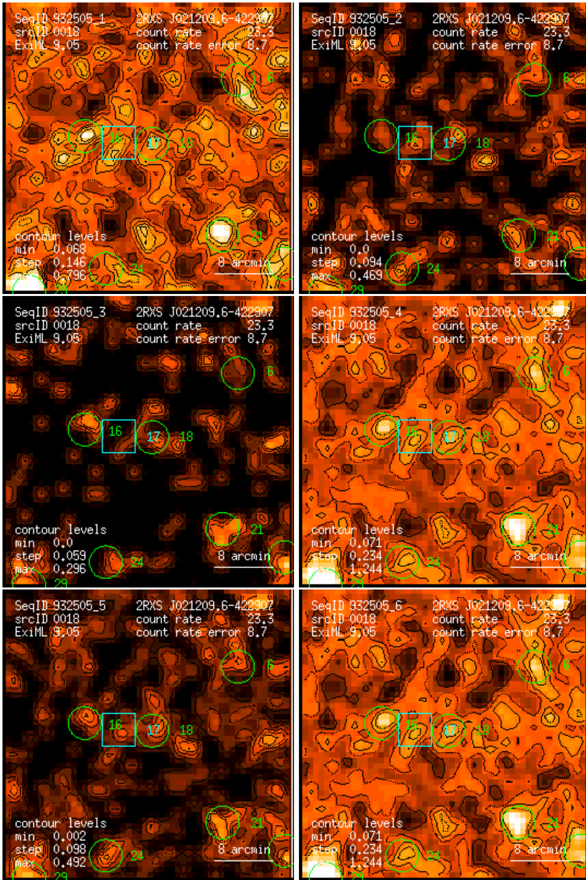
Figure 18: RASS 932505: detection 0018: band rate images, Gaussian filter: (1) PSPC channels 11 – 41, (2) 52 – 90, (3) 91 – 201, (4) 11 – 235, (5) 52 – 201, (6) 11 – 201. Broad band rates in counts/ks. Band rate contour levels in counts/ks/arcmin 2 .
