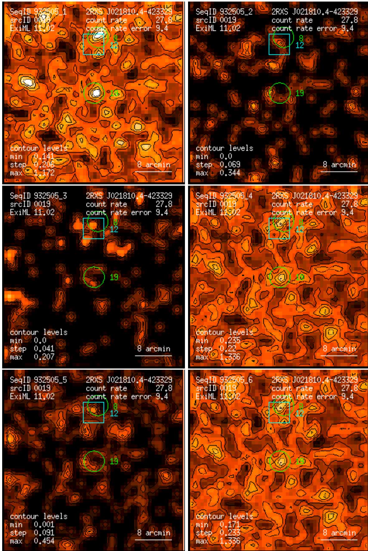
Figure 19: RASS 932505: detection 0019: band rate images, Gaussian filter: (1) PSPC channels 11 – 41, (2) 52 – 90, (3) 91 – 201, (4) 11 – 235, (5) 52 – 201, (6) 11 – 201. Broad band rates in counts/ks. Band rate contour levels in counts/ks/arcmin 2 .
