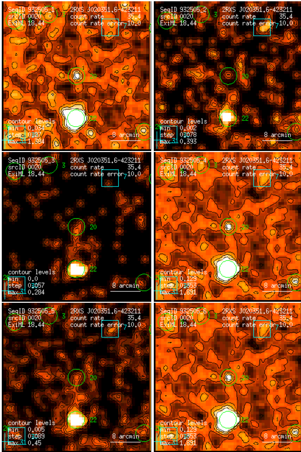
Figure 20: RASS 932505: detection 0020: band rate images, Gaussian filter: (1) PSPC channels 11 – 41, (2) 52 – 90, (3) 91 – 201, (4) 11 – 235, (5) 52 – 201, (6) 11 – 201. Broad band rates in counts/ks. Band rate contour levels in counts/ks/arcmin 2 .
