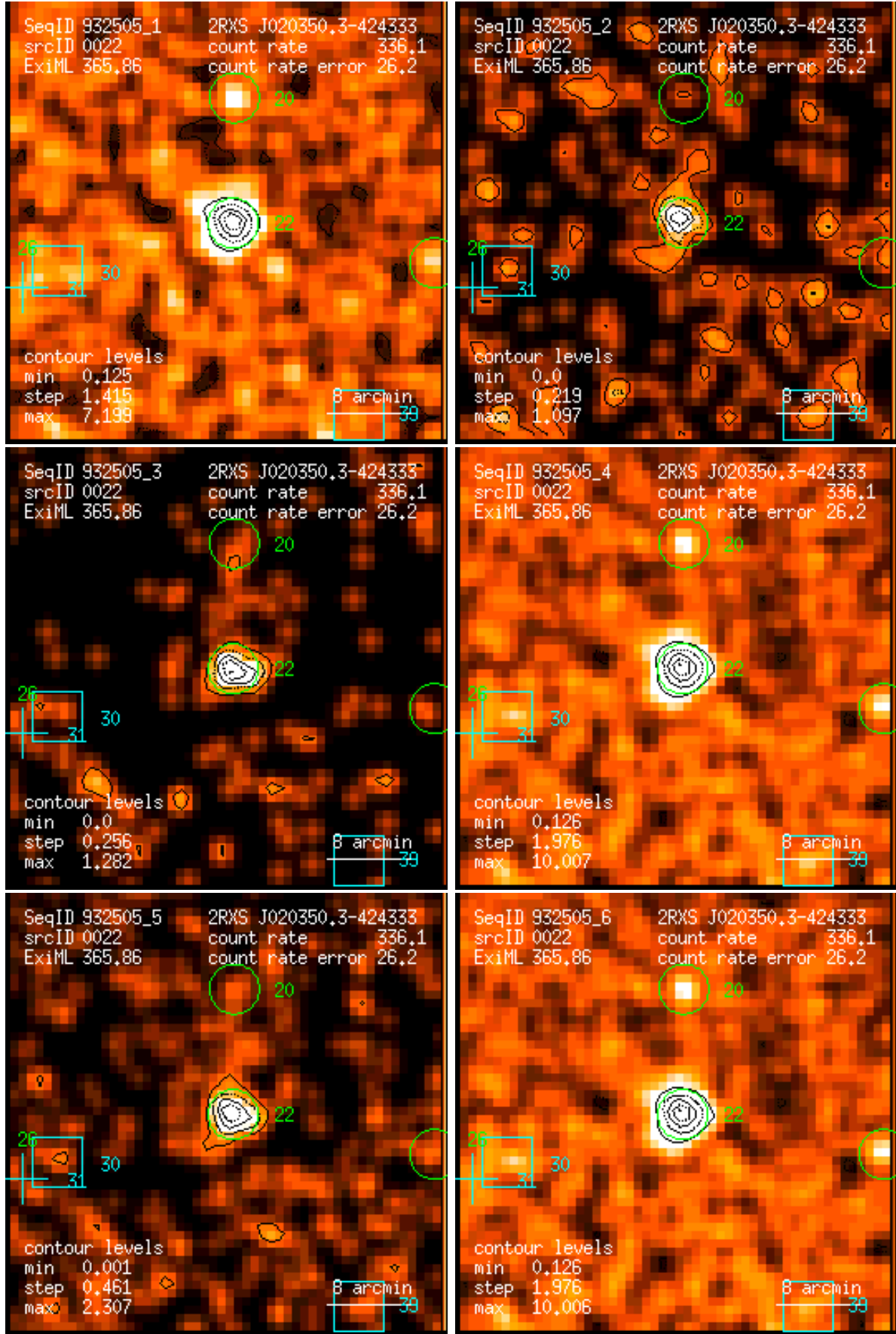
Figure 22: RASS 932505: detection 0022: band rate images, Gaussian filter: (1) PSPC channels 11 – 41, (2) 52 – 90, (3) 91 – 201, (4) 11 – 235, (5) 52 – 201, (6) 11 – 201. Broad band rates in counts/ks. Band rate contour levels in counts/ks/arcmin 2 .
