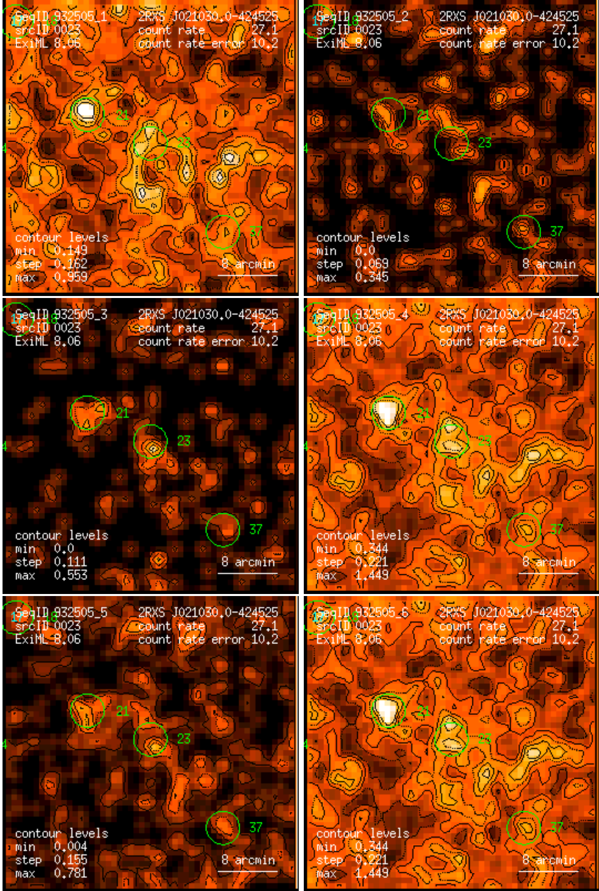
Figure 23: RASS 932505: detection 0023: band rate images, Gaussian filter: (1) PSPC channels 11 – 41, (2) 52 – 90, (3) 91 – 201, (4) 11 – 235, (5) 52 – 201, (6) 11 – 201. Broad band rates in counts/ks. Band rate contour levels in counts/ks/arcmin 2 .
