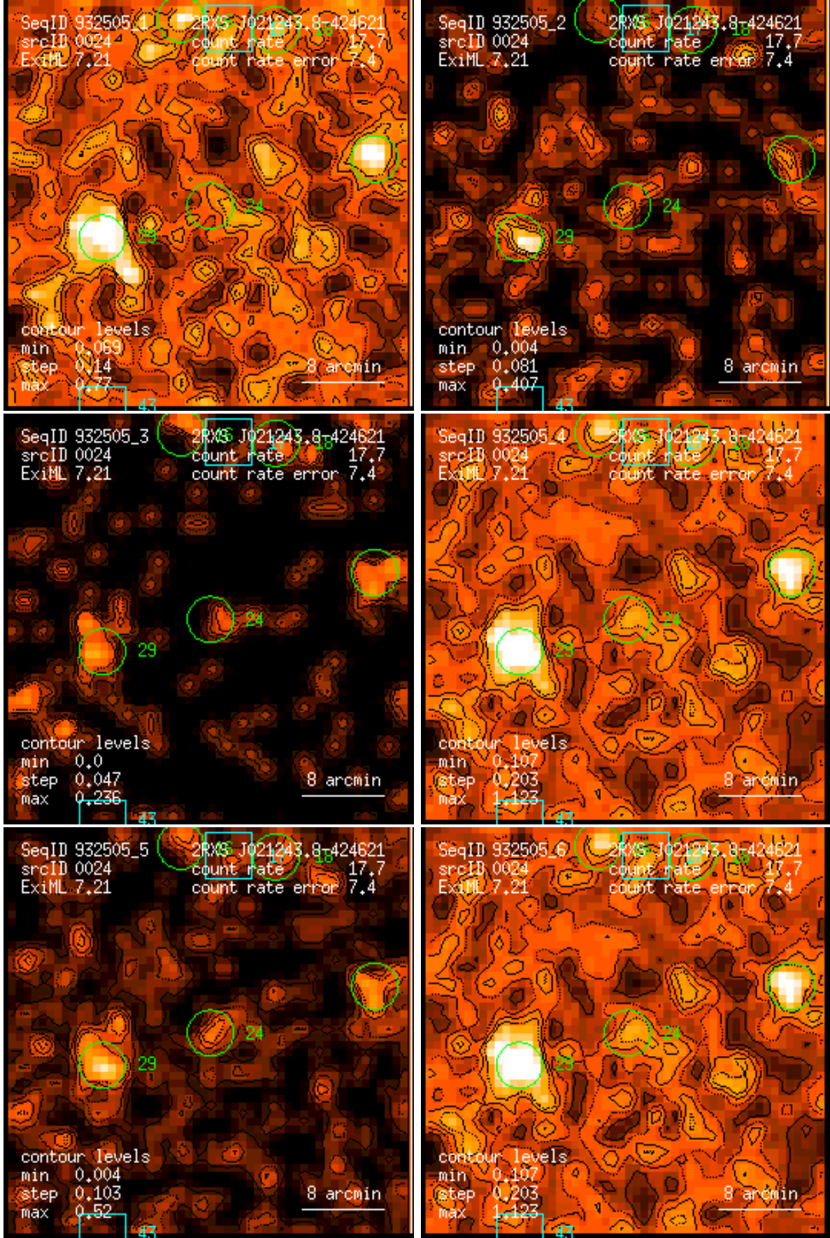
Figure 24: RASS 932505: detection 0024: band rate images, Gaussian filter: (1) PSPC channels 11 – 41, (2) 52 – 90, (3) 91 – 201, (4) 11 – 235, (5) 52 – 201, (6) 11 – 201. Broad band rates in counts/ks. Band rate contour levels in counts/ks/arcmin 2 .
