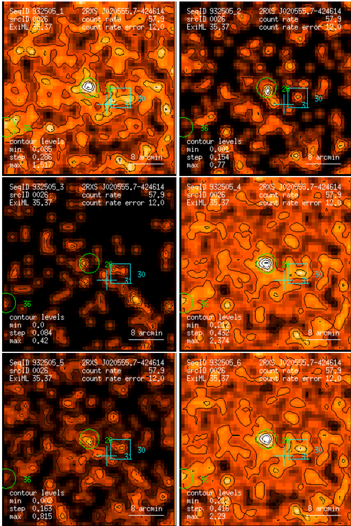
Figure 26: RASS 932505: detection 0026: band rate images, Gaussian filter: (1) PSPC channels 11 – 41, (2) 52 – 90, (3) 91 – 201, (4) 11 – 235, (5) 52 – 201, (6) 11 – 201. Broad band rates in counts/ks. Band rate contour levels in counts/ks/arcmin 2 .
