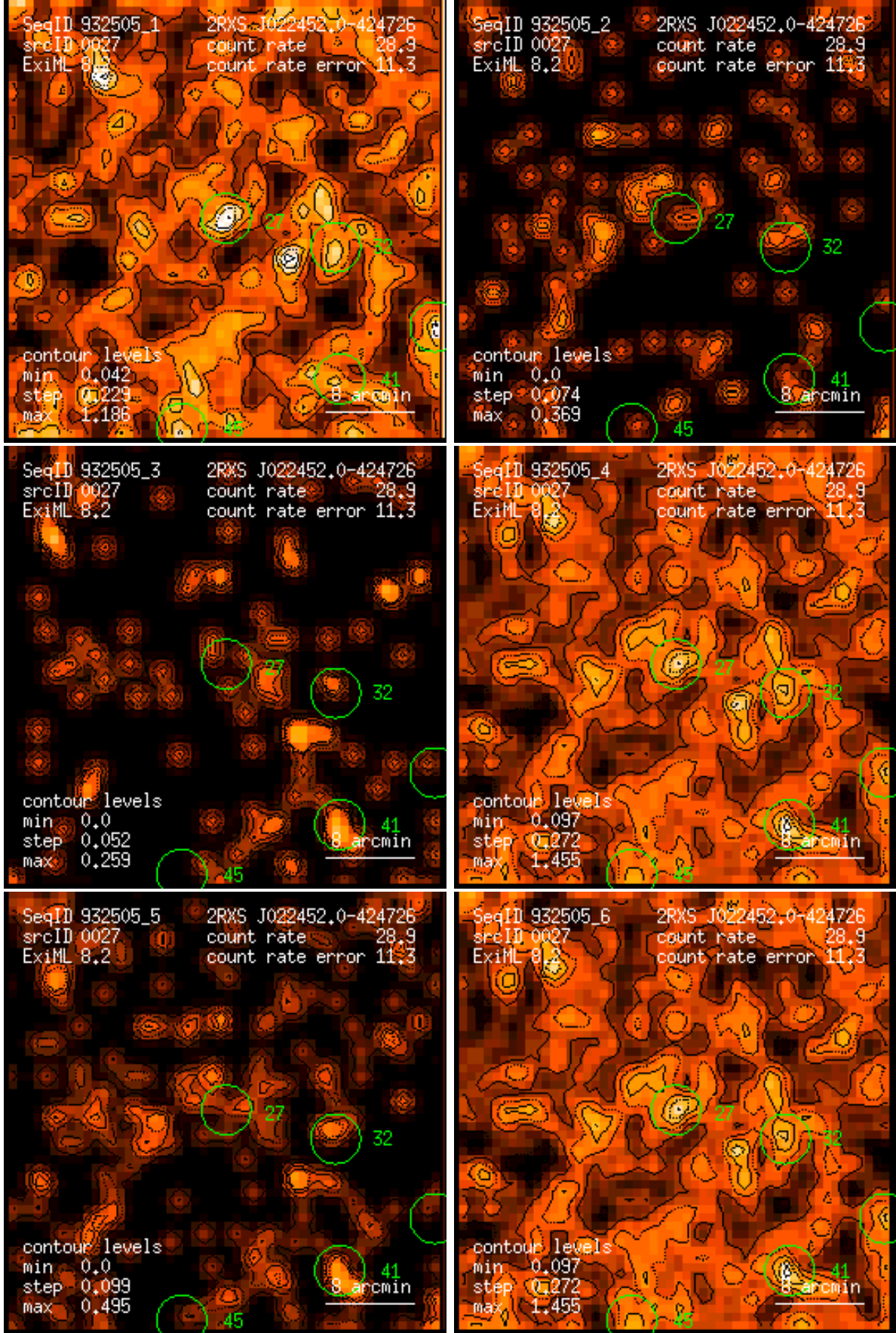
Figure 27: RASS 932505: detection 0027: band rate images, Gaussian filter: (1) PSPC channels 11 – 41, (2) 52 – 90, (3) 91 – 201, (4) 11 – 235, (5) 52 – 201, (6) 11 – 201. Broad band rates in counts/ks. Band rate contour levels in counts/ks/arcmin 2 .
