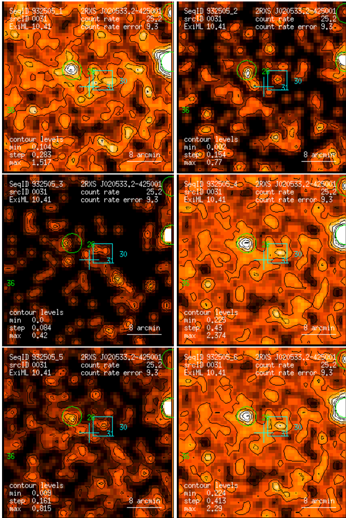
Figure 31: RASS 932505: detection 0031: band rate images, Gaussian filter: (1) PSPC channels 11 – 41, (2) 52 – 90, (3) 91 – 201, (4) 11 – 235, (5) 52 – 201, (6) 11 – 201. Broad band rates in counts/ks. Band rate contour levels in counts/ks/arcmin 2 .
